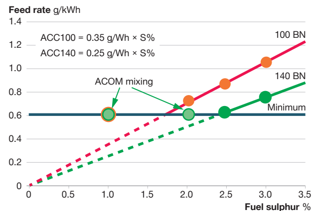
Fig. 3: Feed rate depending on fuel sulphur for a 6G80ME-C9.2 with an FRF = 0.35 g/kWh * %S
