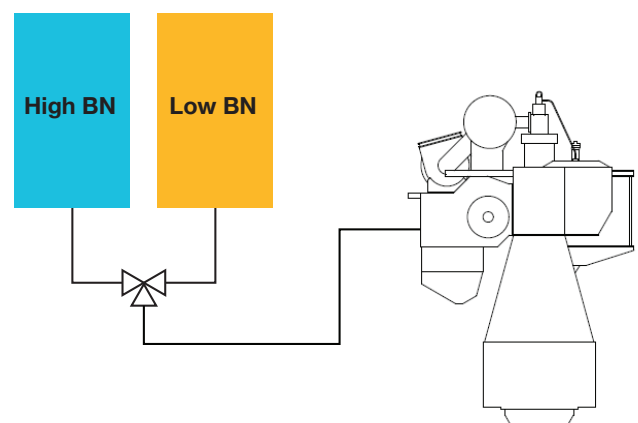
Fig. 2: ACOS: automated cylinder oil switch system
