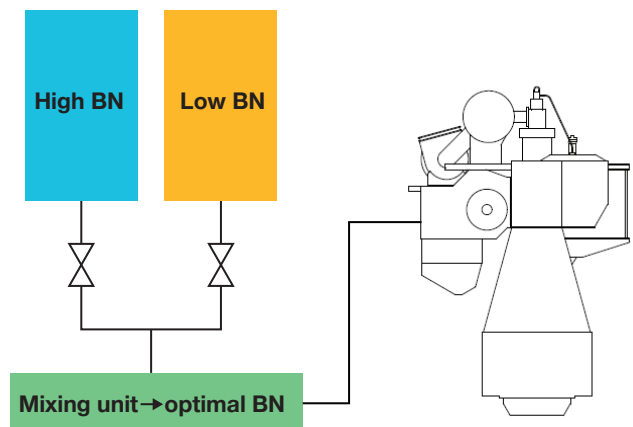
Fig. 1: ACOM: automated cylinder oil mixing system
