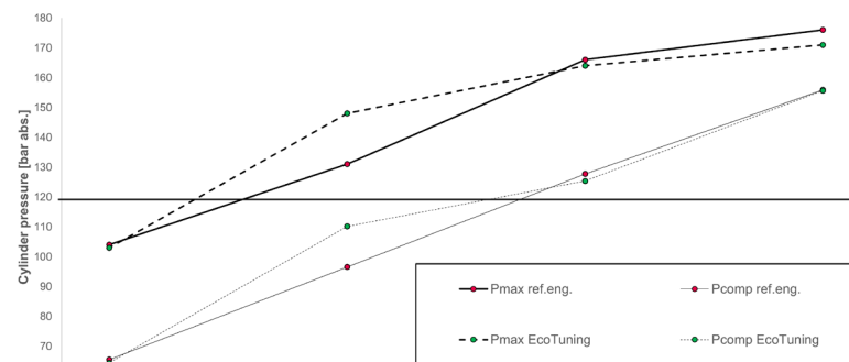
Figure 1: MAN EcoTuning cylinder pressure vs. engine load
