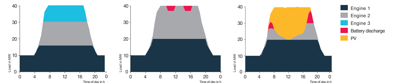
Engines operating at partial-load to meet the reserve requirements.
