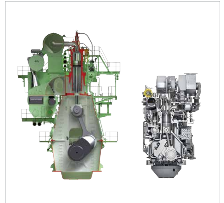
Fig. 3.01: Two-stroke crosshead engine and four-stroke trunk engine, not to scale
