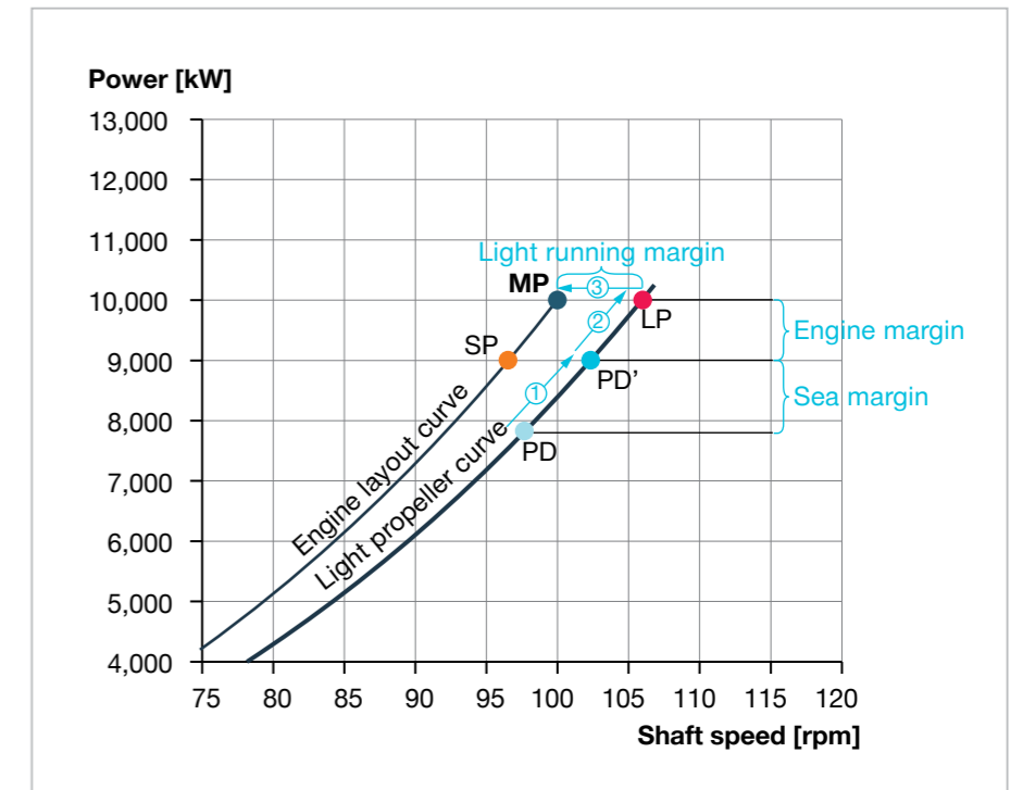
Fig. 3.04: Light propeller curve with added margins resulting in the engine layout curve
