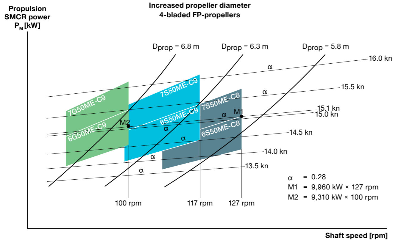
Fig. 3.15: Example of constant ship speed curves with selected engine layout diagrams
