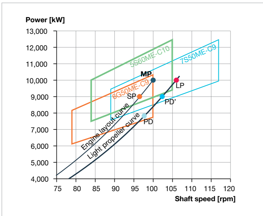
Fig. 3.08: Engine layout diagrams of selected possible engines, see the engine programme
