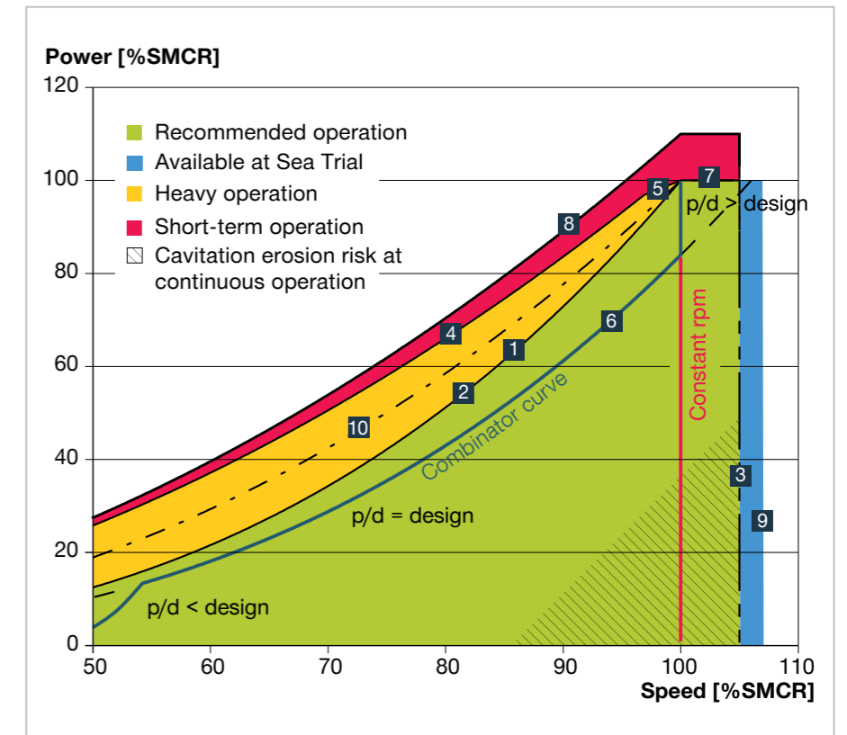
Fig. 3.13: Combinator curve with engine load diagram, see Ref. [3.3]. The constant rpm curve can also be referred to as the generator curve
