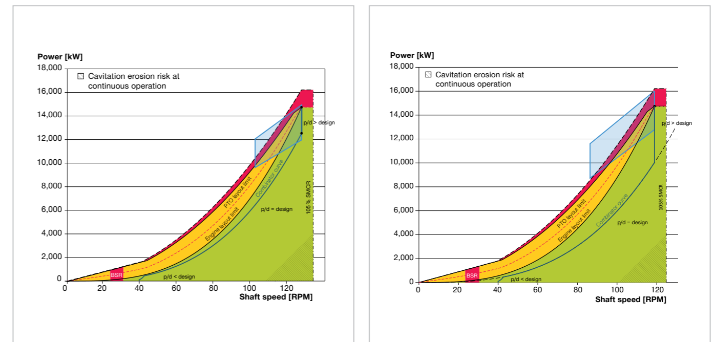
Fig. 5.06: The light propeller curve with conceptual combinator curves plotted on engine load diagram with the layout diagram of the S50ME-C8-GI and S50ME-C9-GI respectively
