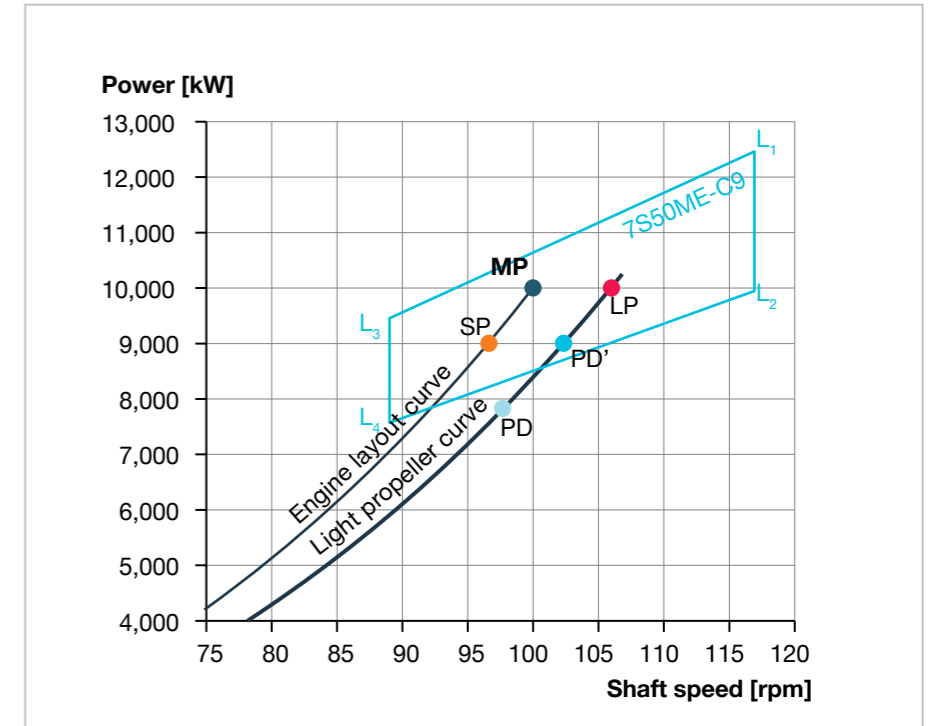
Fig. 3.06: Engine layout diagram with light propeller curve and engine layout curve
