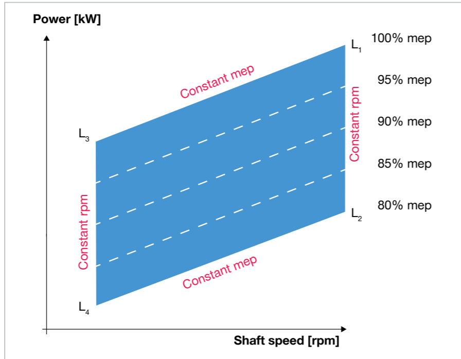
Fig. 3.05: Engine layout diagram with lines of constant mep and rpm
