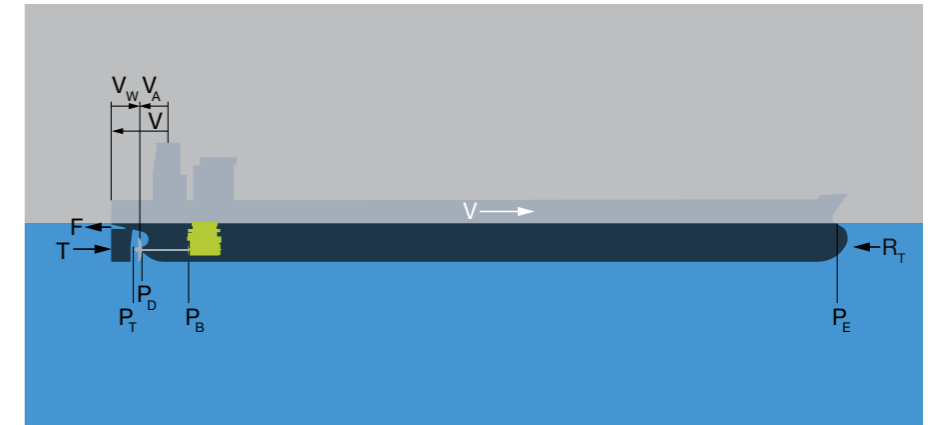
Fig. 2.06: Propulsion power
