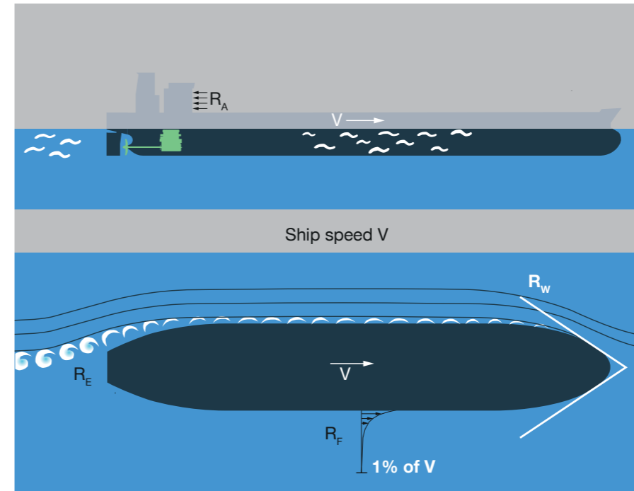
Fig. 1.04: Components of resistance on a ship
