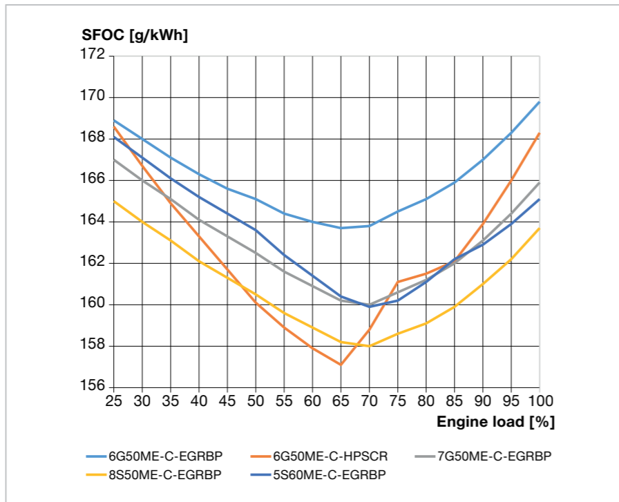
Fig. 5.02: SFOC values of possible engines for a 50,000 dwt MR tanker in Tier III mode with a scrubber installed and a SMCR of 8,900 kW at 93 rpm, as of 2018. Values may change, please use CEAS for specific values
