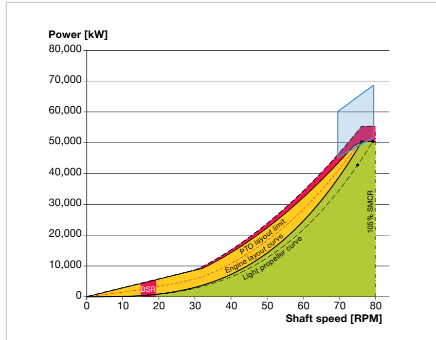
Fig. 5.04: Engine load diagram with PTO layout limit and layout diagram of the 10G95ME-C10-EGRTC
