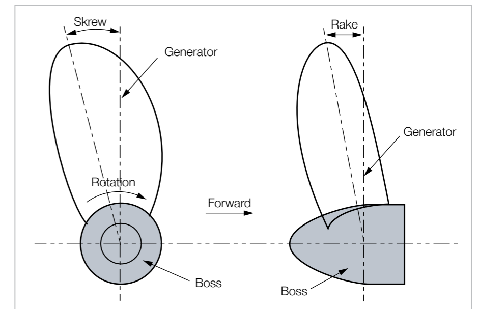
Fig. 2.04: Rake and skew
