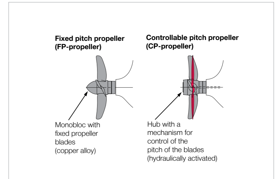
Fig. 2.03: Propeller types
