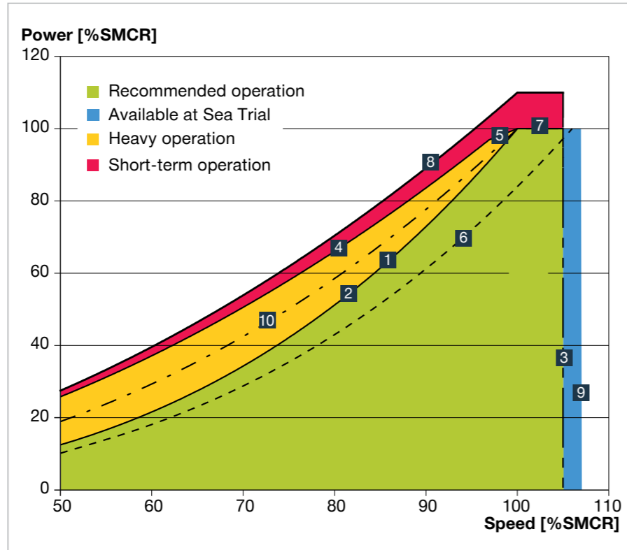
Fig. 3.10: Engine load diagram with marked lines
