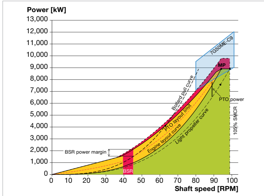
Fig. 5.01: Light propeller curve, margins and layout curve for SMCR = 8,900 kW with load diagram and layout diagram for a potential engine for a 50,000 dwt MR tanker. Maximum available PTO power at 75% MCR is approx. 1,250 kW
