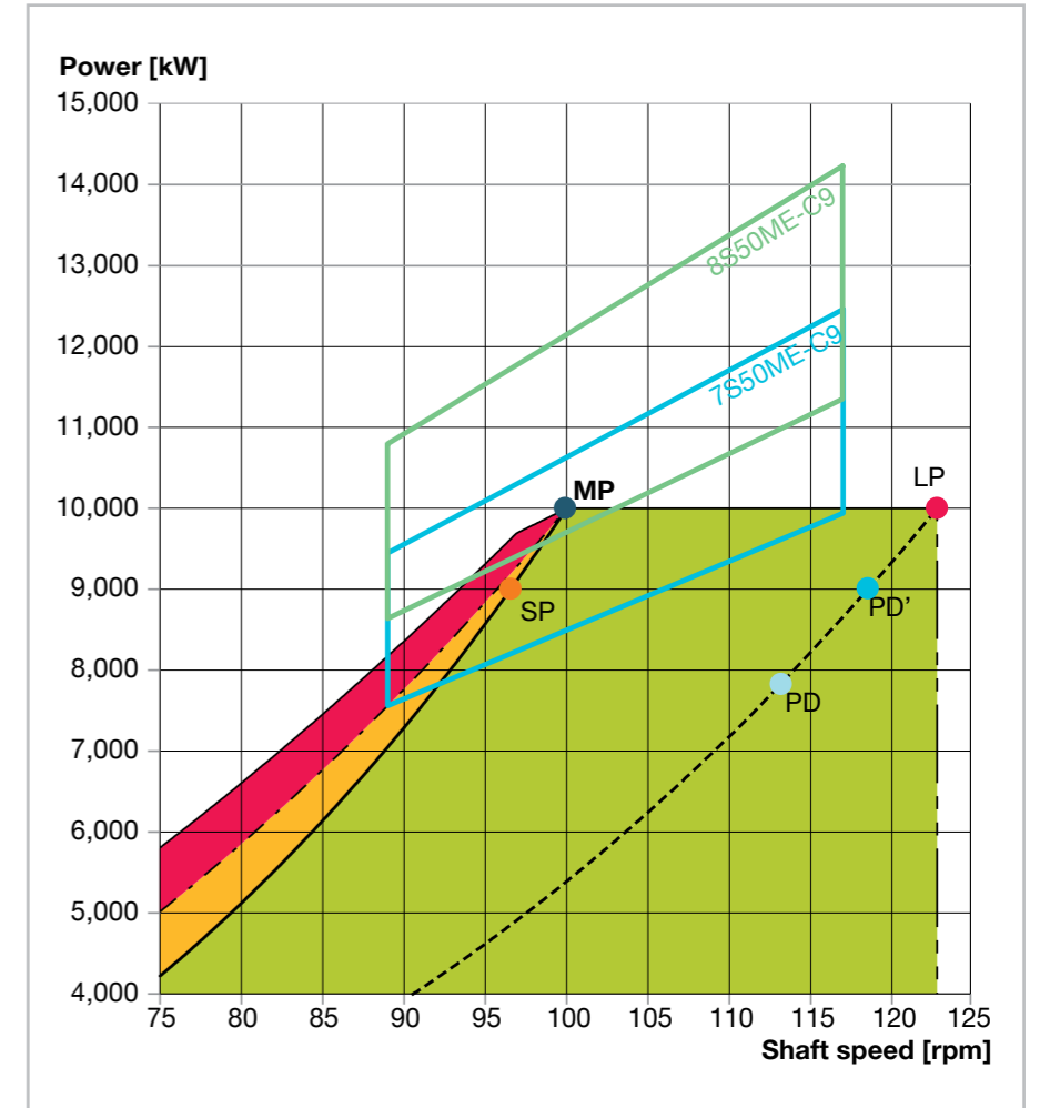
Fig. 3.14: Rpm extended load diagram, for an extreme case
