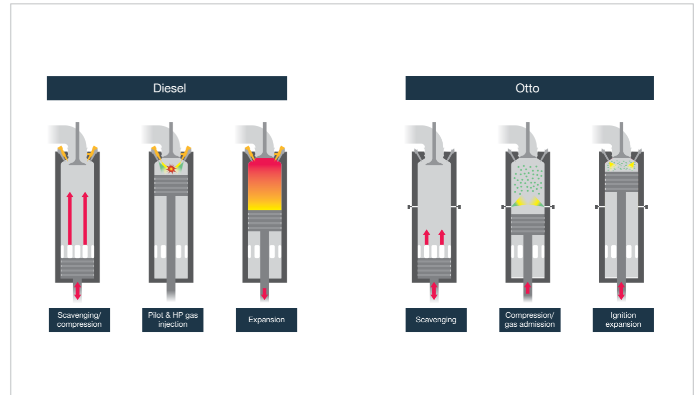
Fig. 3.02: Diesel and otto cycles for dual fuel engines
