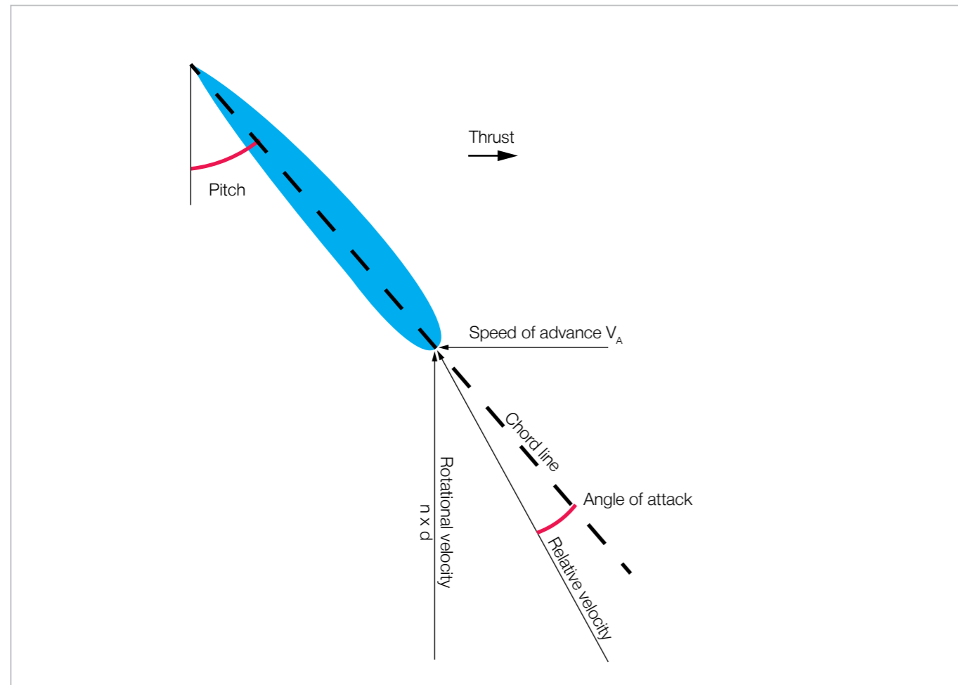
Fig. 2.07: Advance number
