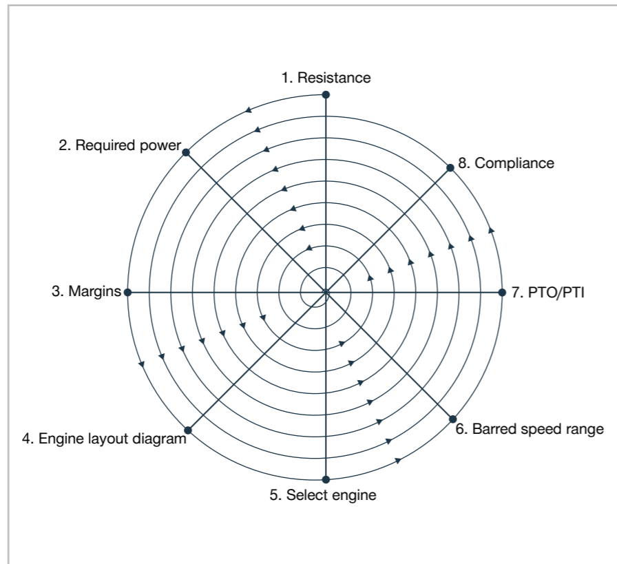
Fig. 3.03: FPP engine selection spiral
