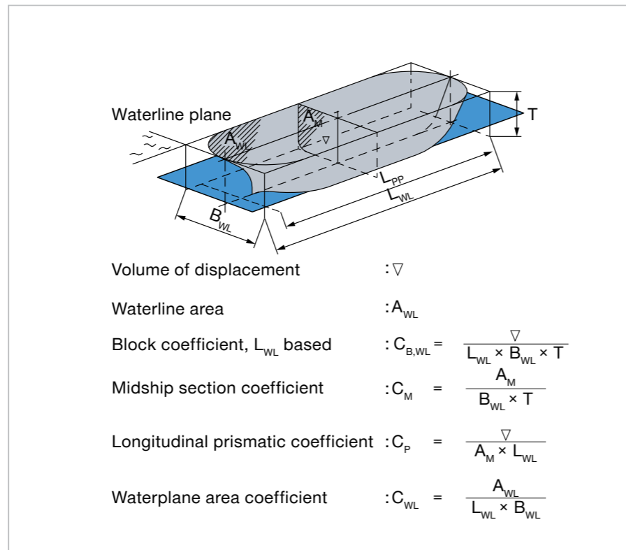
Fig. 1.02: Hull coefficients
