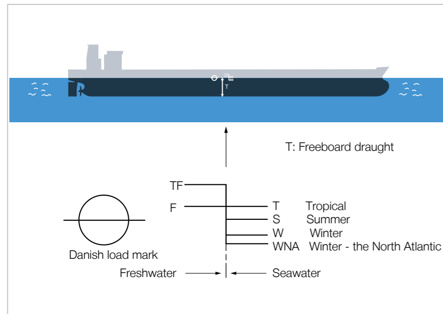
Fig. 1.03: Load lines
