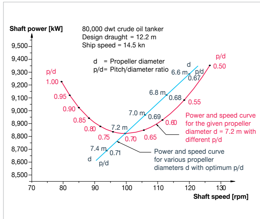
Fig. 2.09: Example of influence of diameter and pitch
