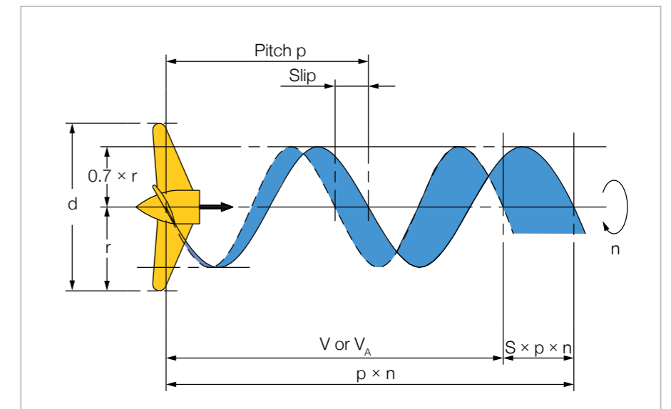
Fig. 2.01: Propeller pitch and slip
