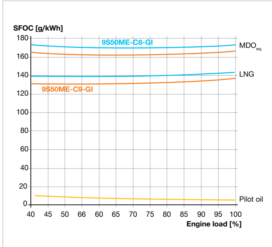
Fig. 5.07: SFOC along the possible combinator curves shown in Fig. 5.06 for Tier III mode. MDO equivalents, LNG, and pilot oil consumption (similar for both engines) are shown separately
