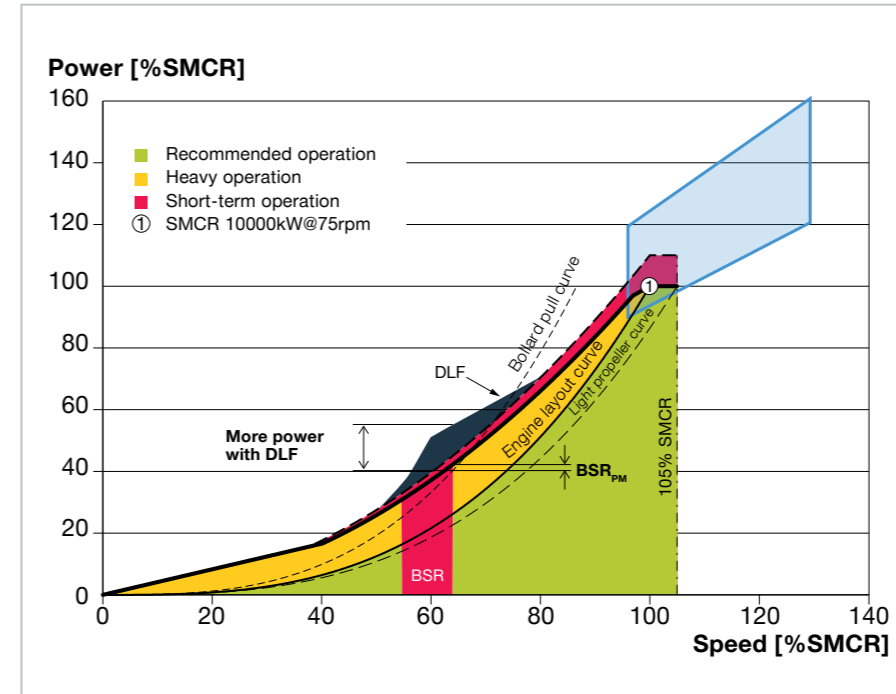
Fig. 3.09: An example of a BSR extending above 60% rpm and resulting small BSR PM . In this example DLF was applied as a retrofit to reduce BSR passage time
