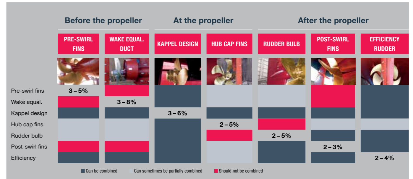
Fig. 2.10: Possibilities for combining energy saving devices, including individual saving potential
