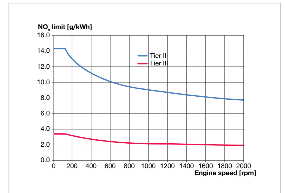
Fig. 4.03: Limits on NO x emissions depending on engine speed
