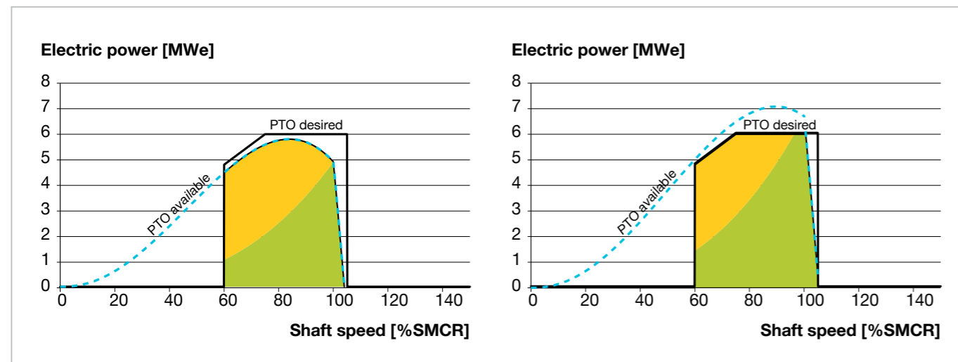
Fig. 5.05: PTO availability over the full speed range with the original (left) and increased SMCR (right)
