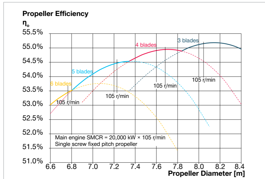
Fig. 2.02: Propeller efficiency and blade number. Notice that rpm is constant and therefore the diameter must be increased to achieve optimum
