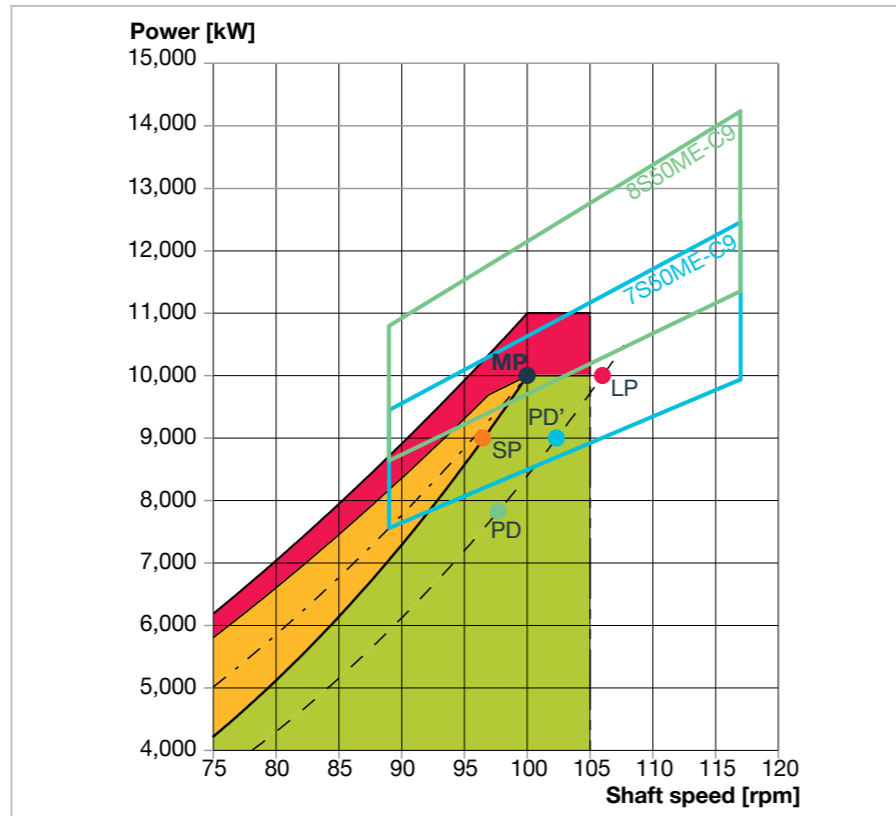
Fig 3.11: Engine load diagram , with different layout diagrams , note that the appearance of the load diagram is independent of the position of point MP within a layout diagram
