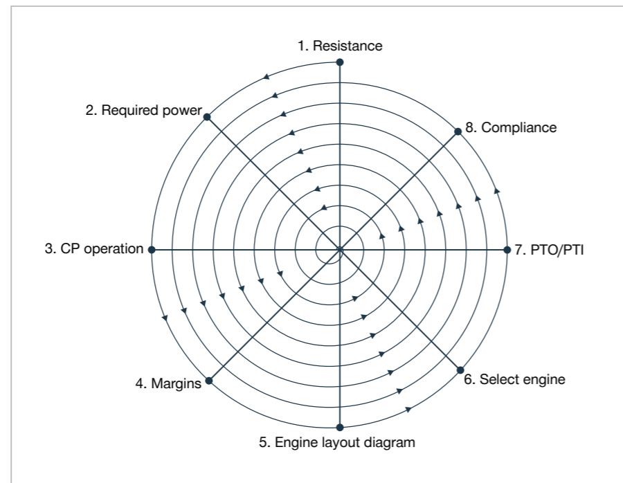
Fig. 3.12: CPP engine selection spiral
