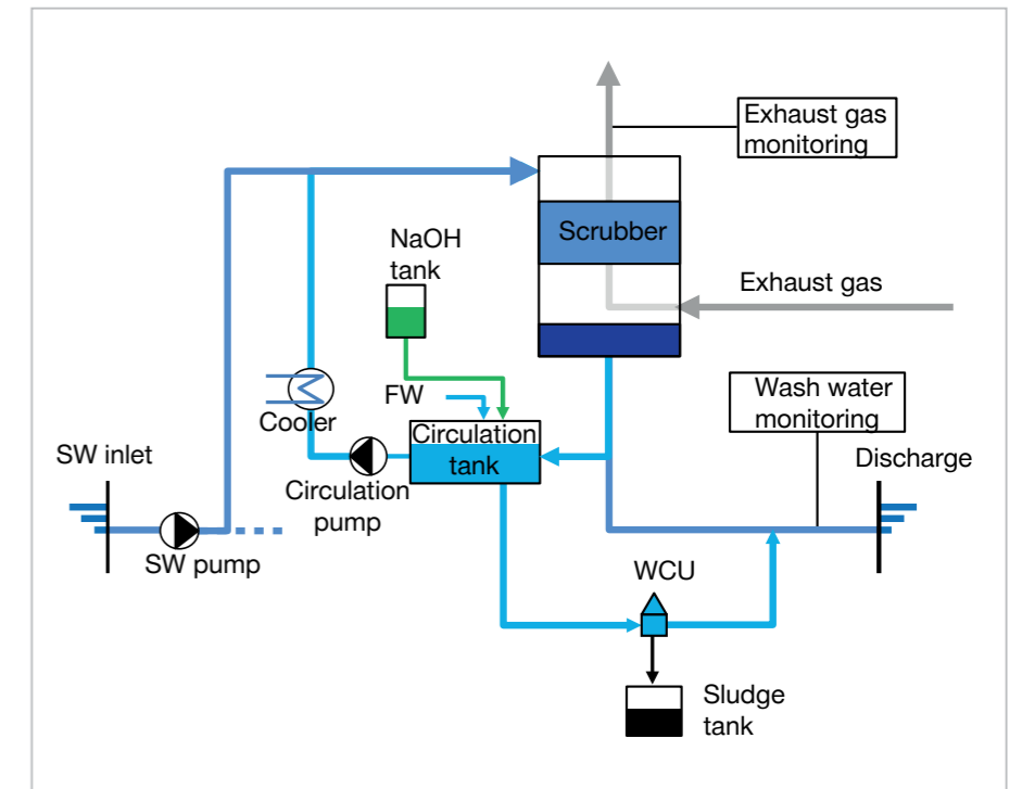
Fig. 4.02: Hybrid scrubber system
