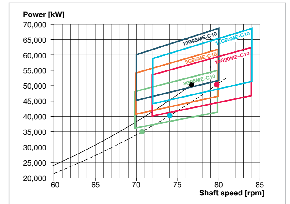
Fig. 5.03: Layout diagrams for selected engines possible for the example 19,000 teu container carrier
