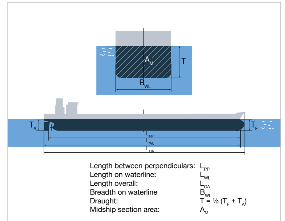
Fig. 1.01: Hull dimensions
