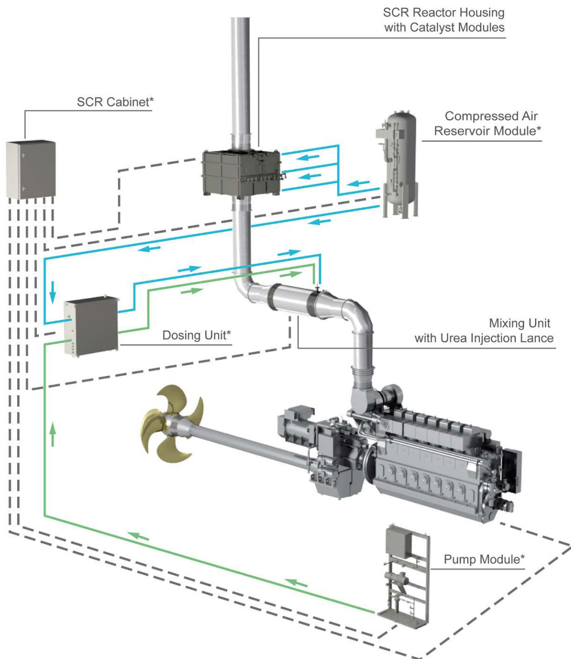
Figure 6: SCR system components overview (example)
