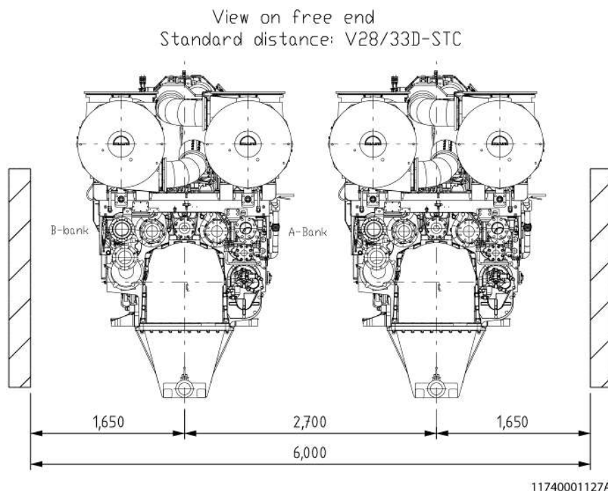
Figure 105: Space requirement for maintenance
