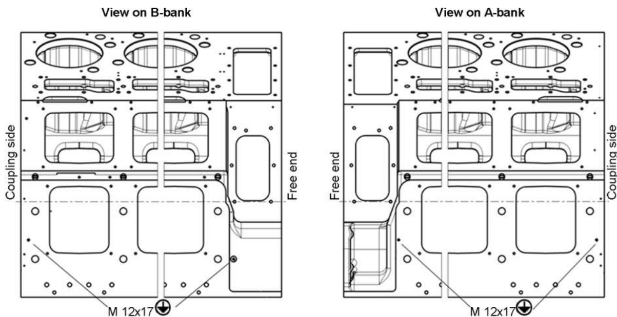
Figure 24: Earthing connection on engine
