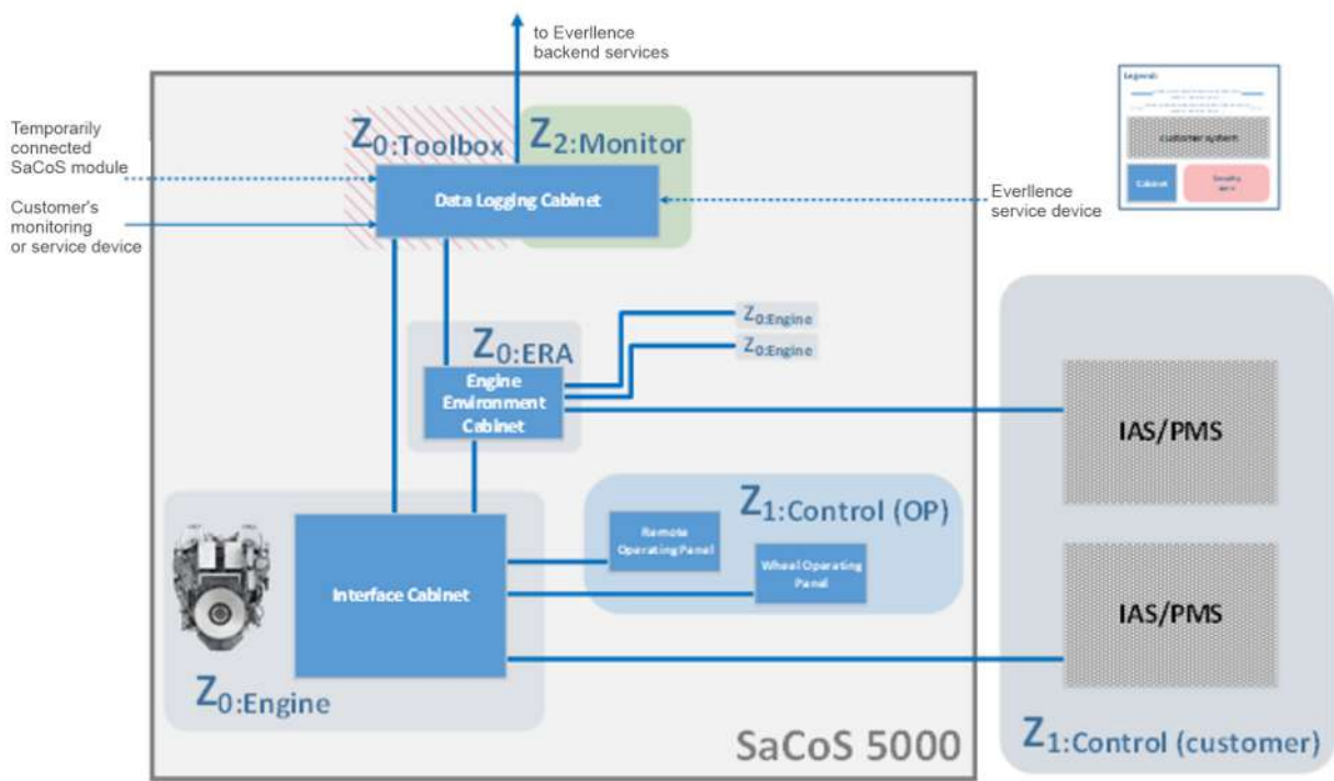
Figure 77: SaCoS 5000 Largebore with SCR and EngineVault: Zones and connections (simplified)
