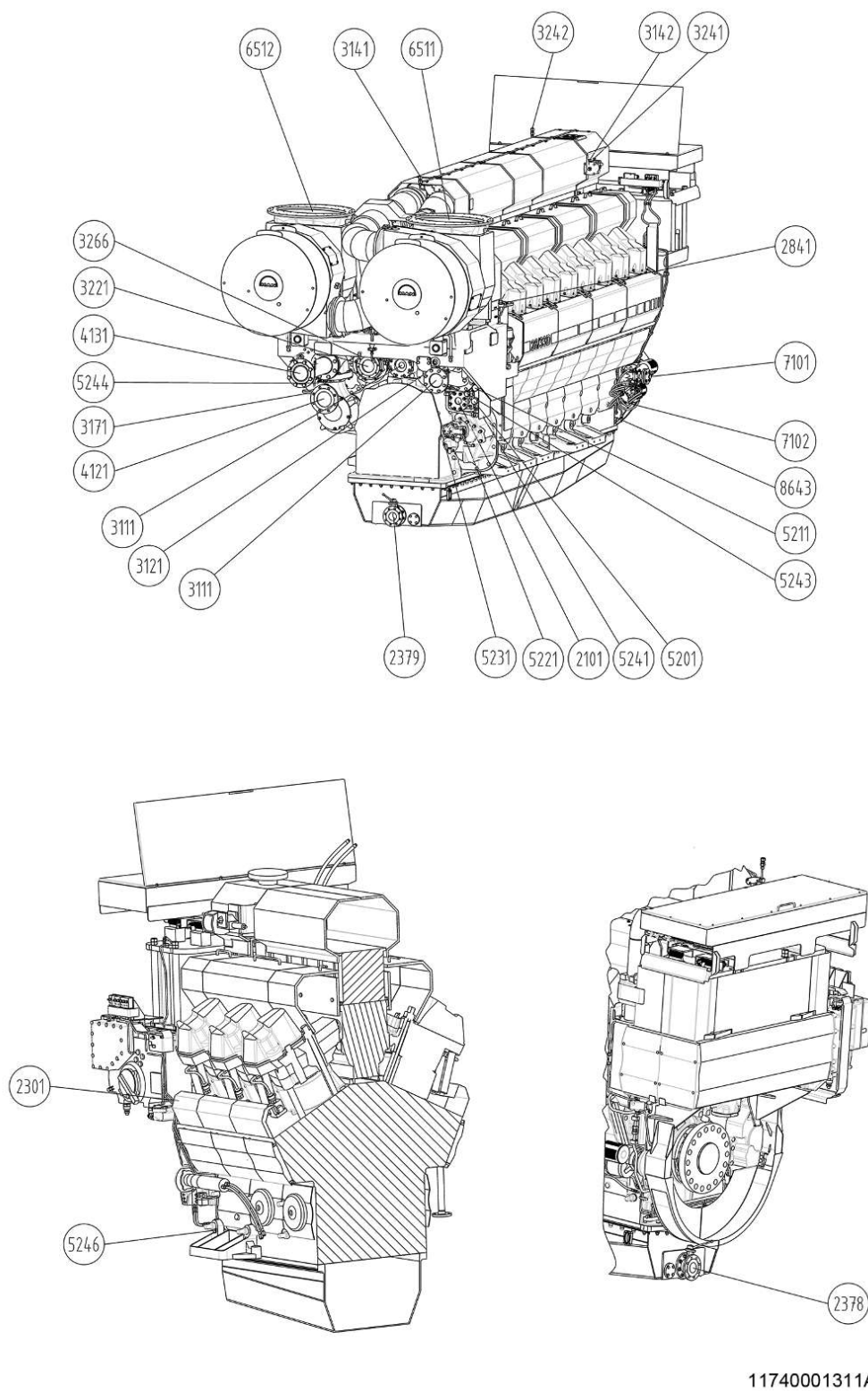
Figure 67: Engine pipe connections
