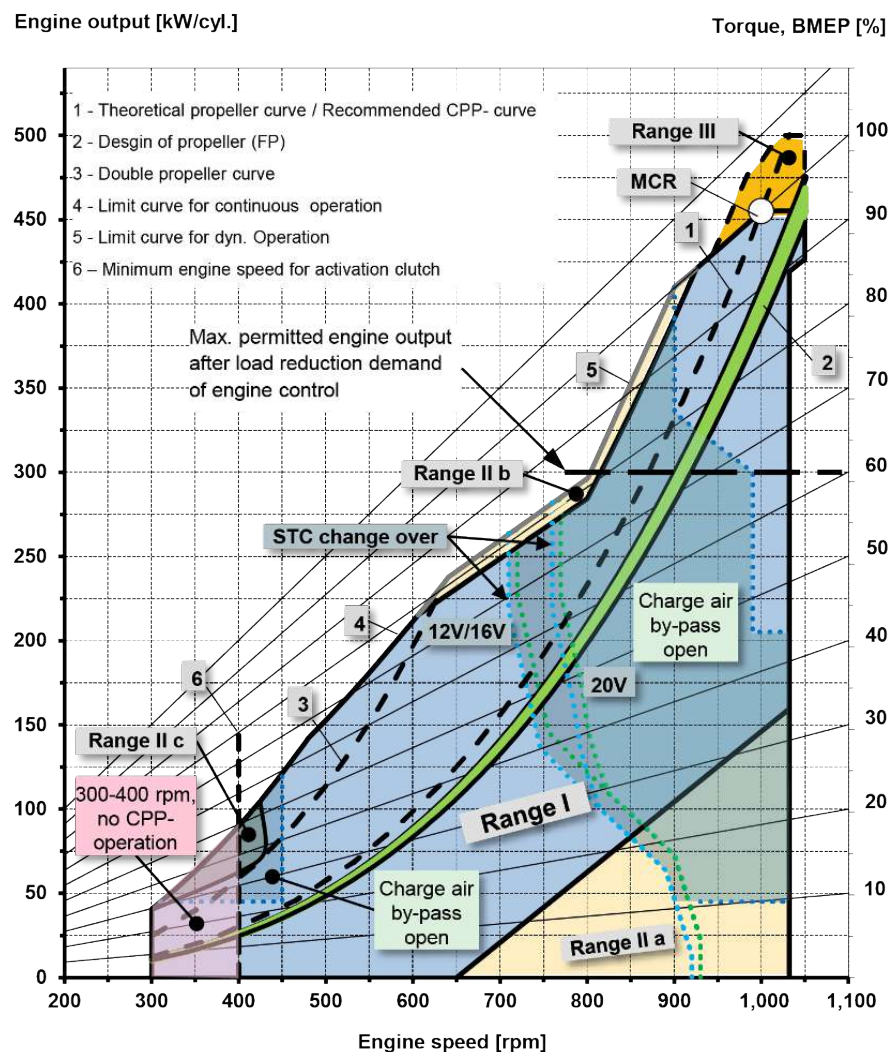
Figure 25: STC operating range for mechanical propulsion (FPP, water jet, CPP)
