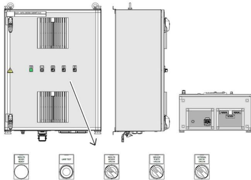
Figure 46: Data Logging Cabinet Plus (DLC+)
