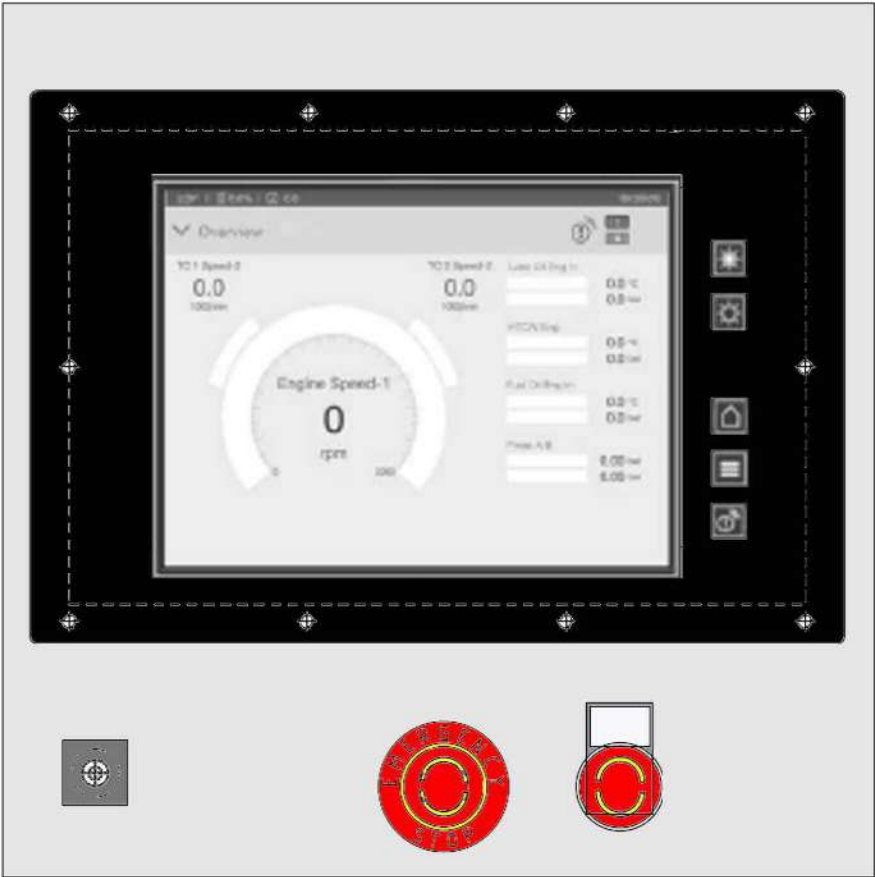
Figure 57: Wheelhouse Operating Panel
