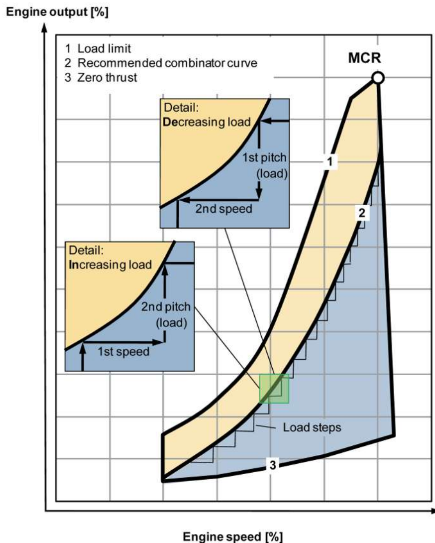
Figure 26: Example to illustrate the change from one load step to another
