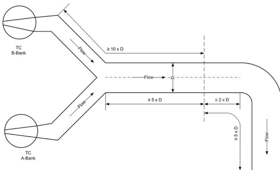
Figure 34: Position of sampling points (exemplary)
