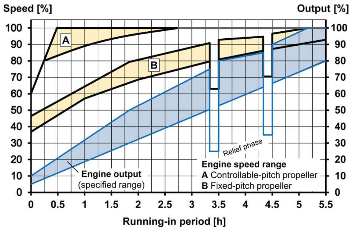
Figure 116: Standard running-in programme for marine engines (variable speed)
