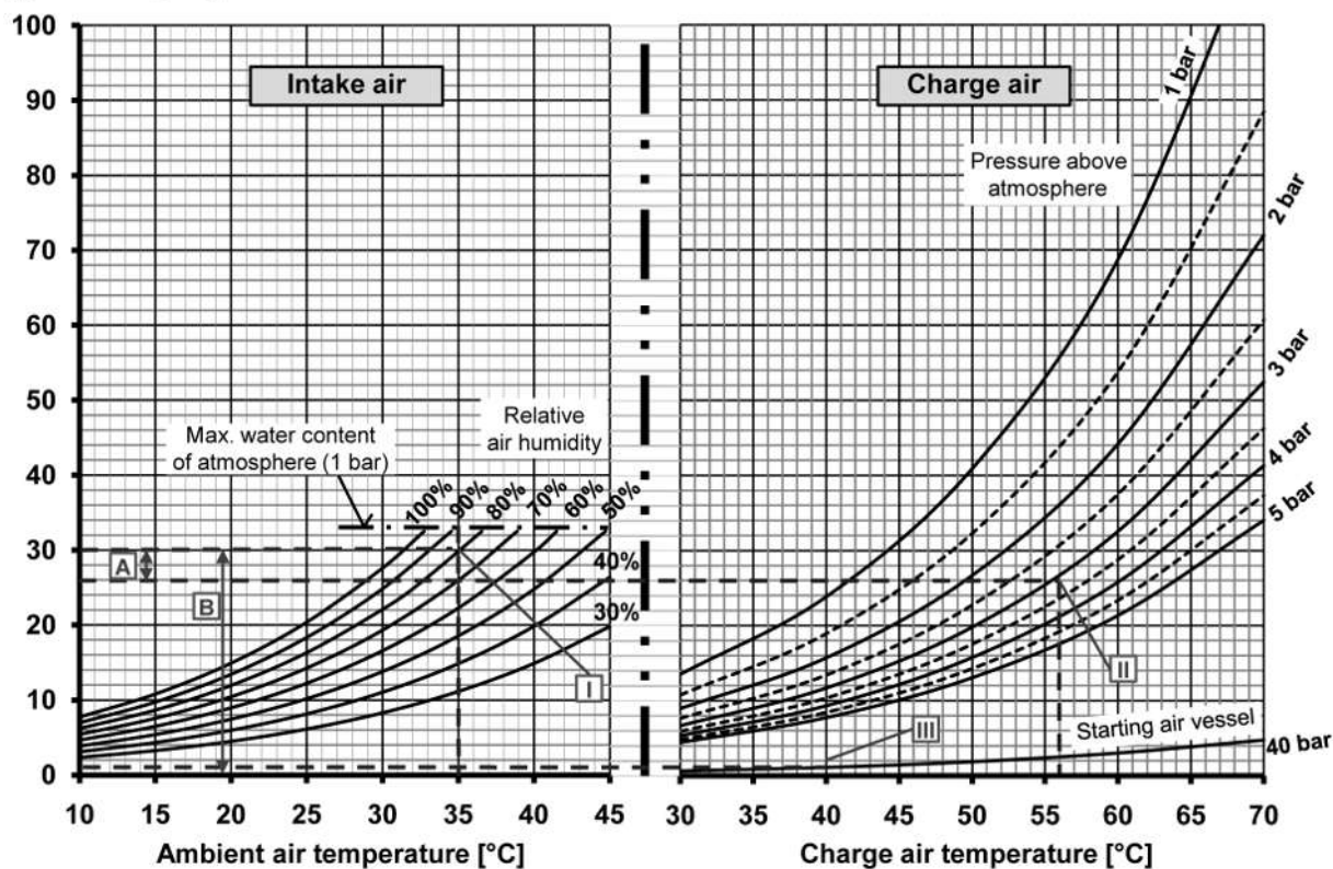
Figure 74: Diagram condensate amount
