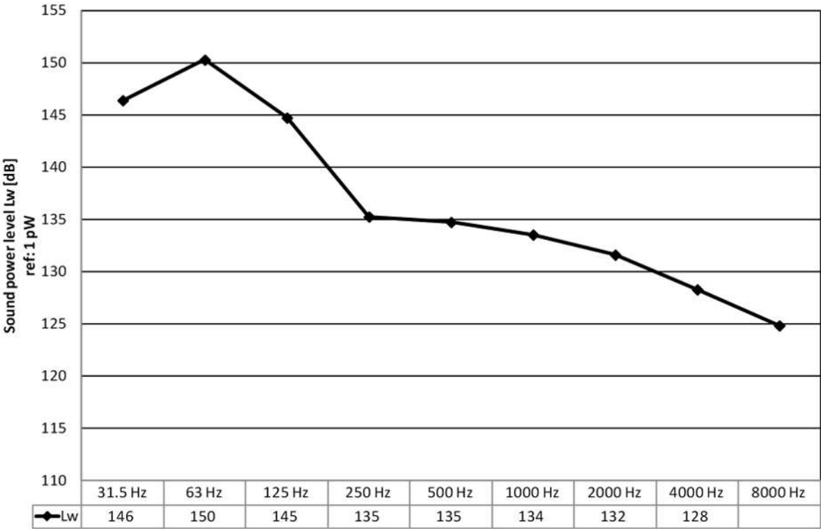
Figure 38: Unsilenced exhaust gas noise – Sound power level Lw – Octave level diagram
