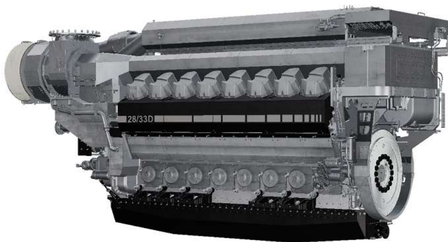
Figure 8: Engine overview, lube oil module with automatic filter, engine view on coupling side (CS)
