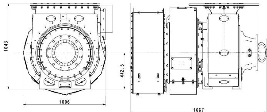
Figure 104: Exemplary illustration of TCA33
