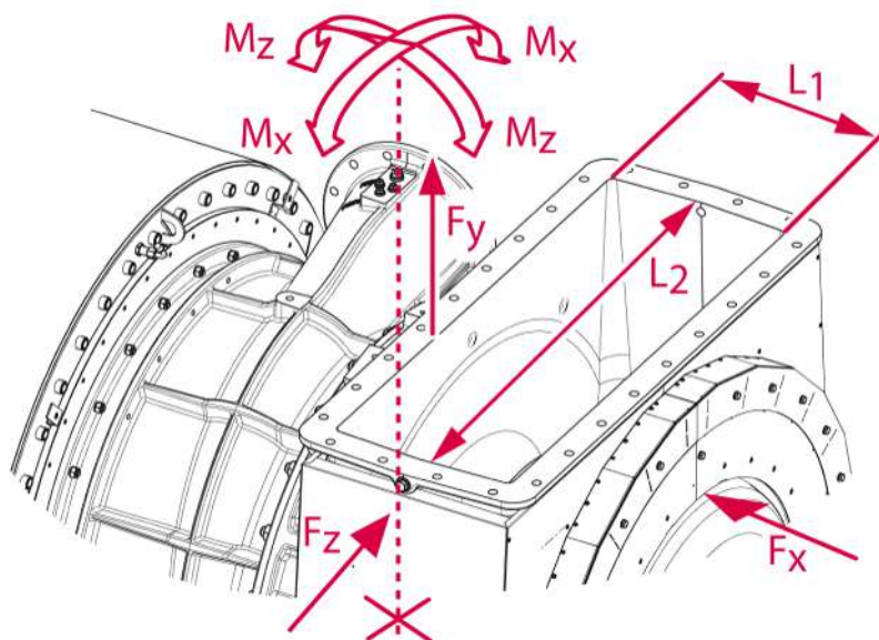
Figure 11: Maximum connection loads on gas outlet casing
