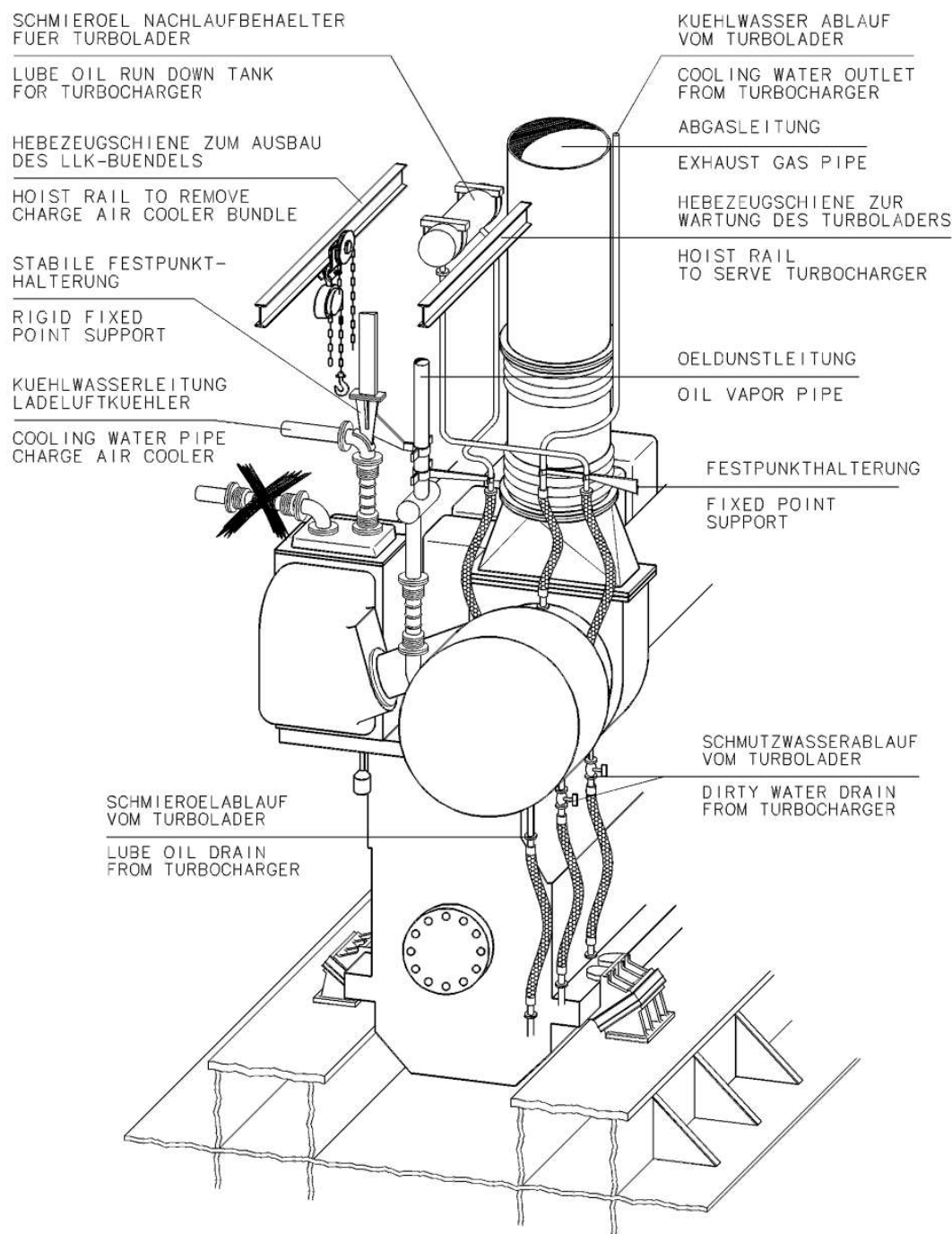
Figure 71: Installation of hoses
