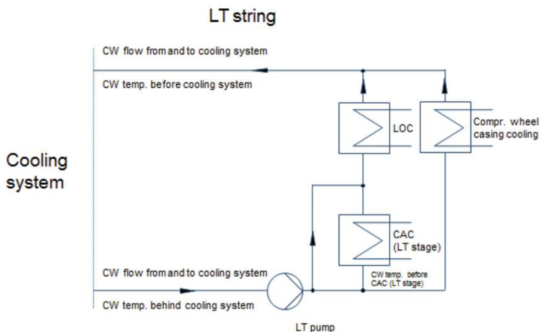
Figure 32: Flow scheme LT string
