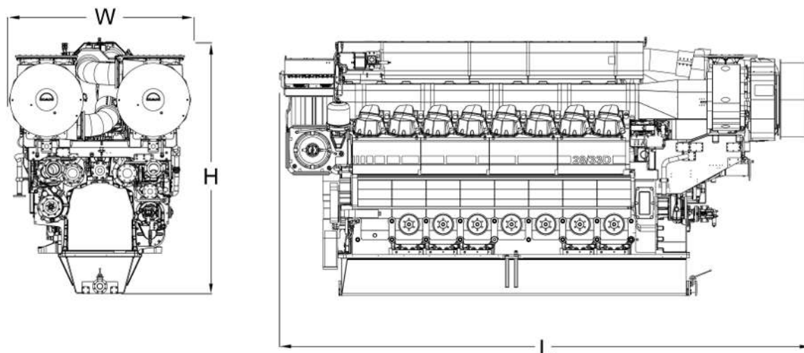
Figure 13: Main dimensions and weights – V28/33D STC mechanical propulsion (lube oil module with automatic filter)
