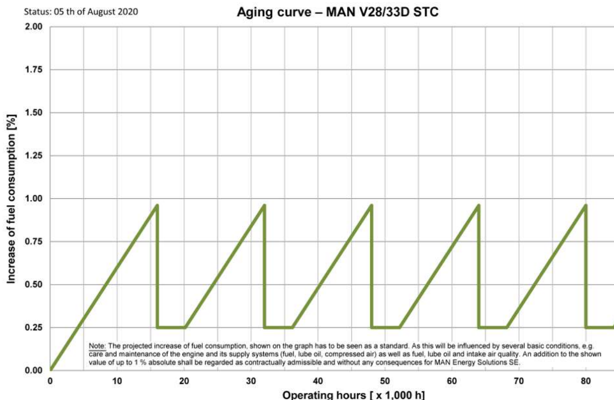
Figure 28: Influence of total engine running time and service intervals on fuel oil consumption
