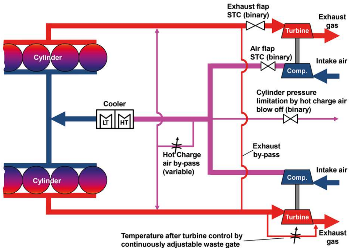
Figure 18: Overview flaps
