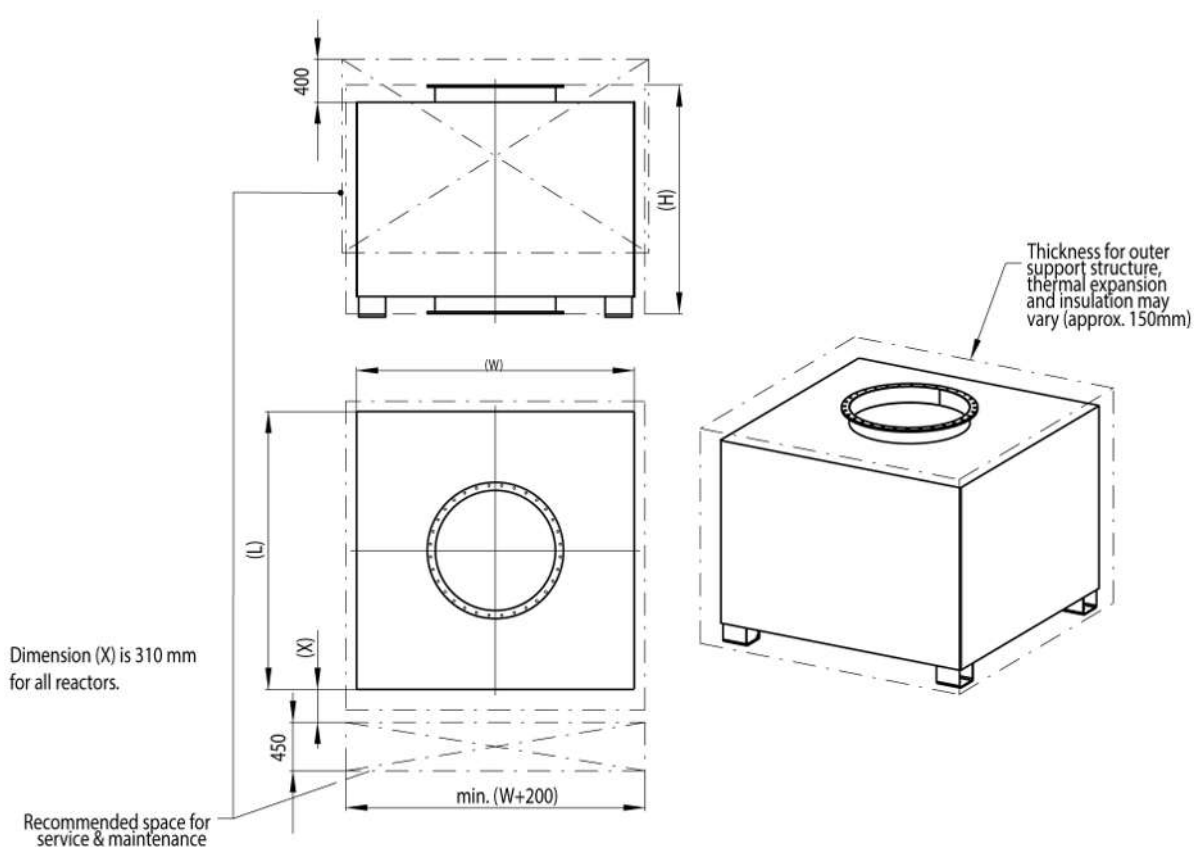
Figure 15: SCR reactor
