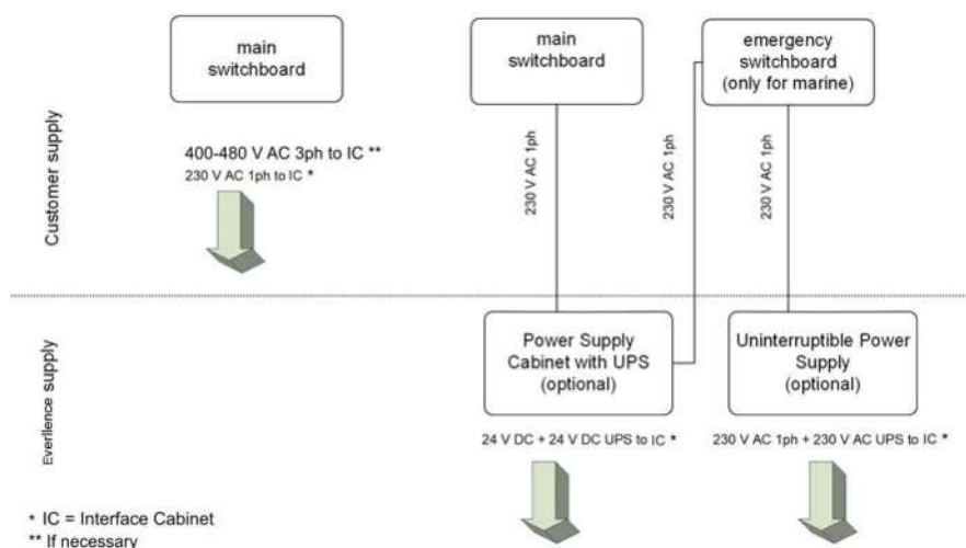
Figure 60: Supply diagram with Power Supply Cabinet and UPS
