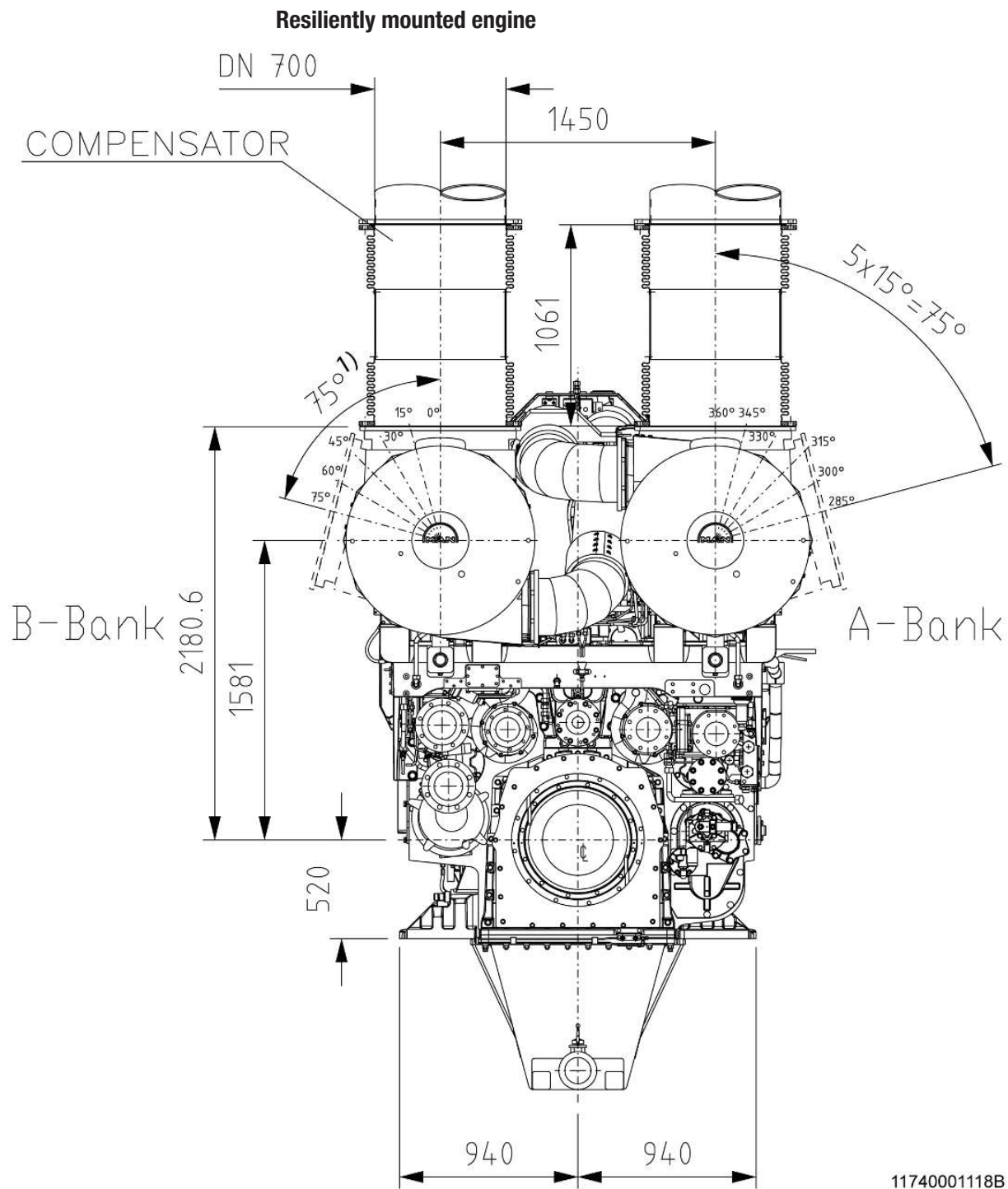
Figure 108: Possible positions of the outlet casing of the turbocharger – View on counter coupling side
