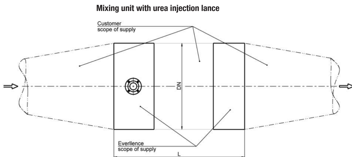
Figure 16: Mixing unit with urea injection lance
