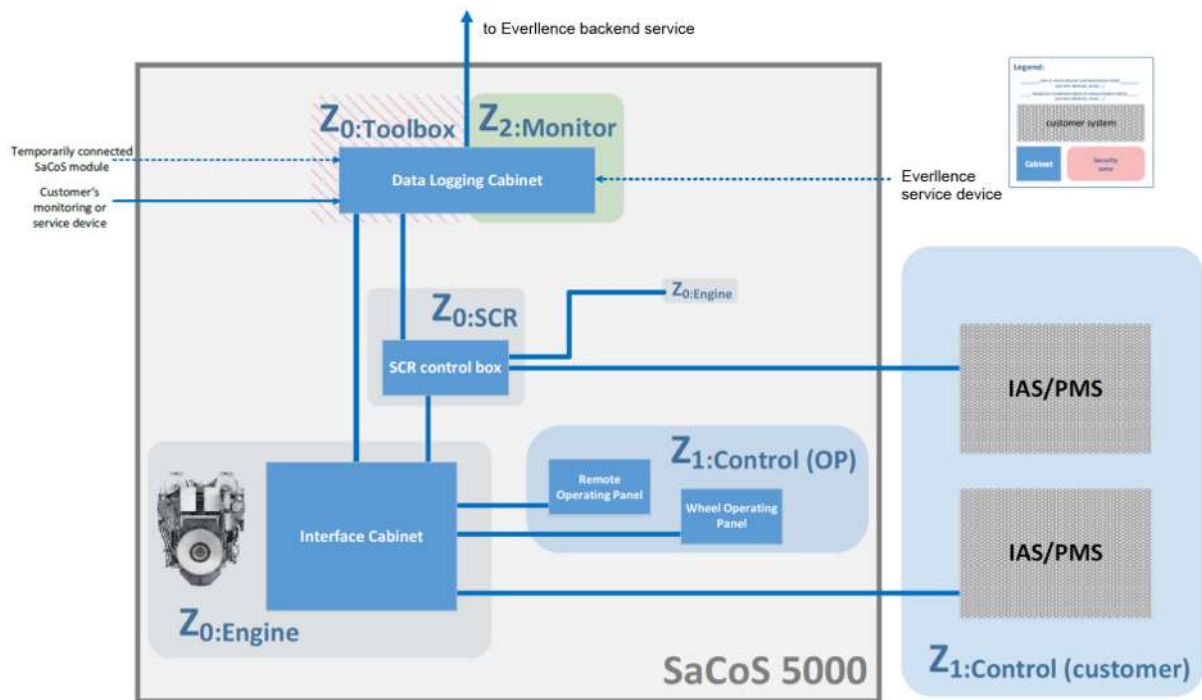
Figure 48: SaCoS 5000 with SCR and DLC: Zones and connections (simplified)
