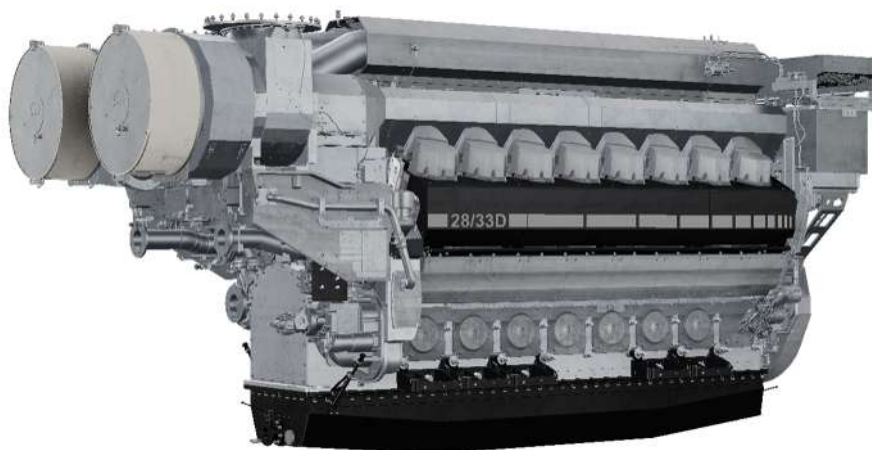
Figure 7: Engine overview, engine view on counter coupling side (CCS)
