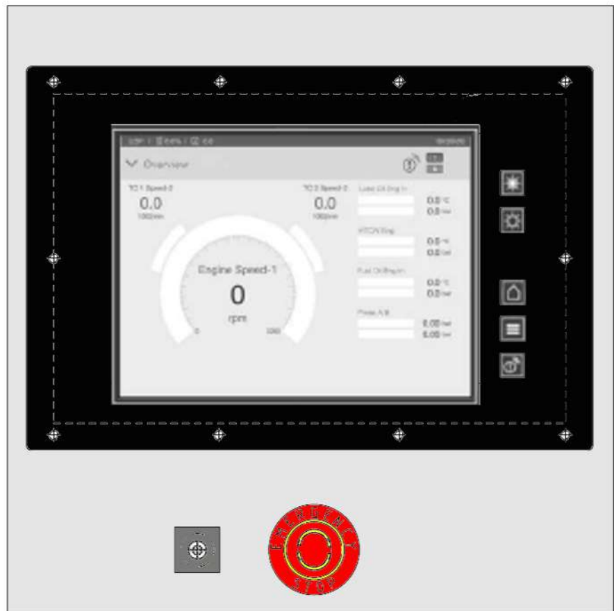
Figure 56: Remote Operating Panel
