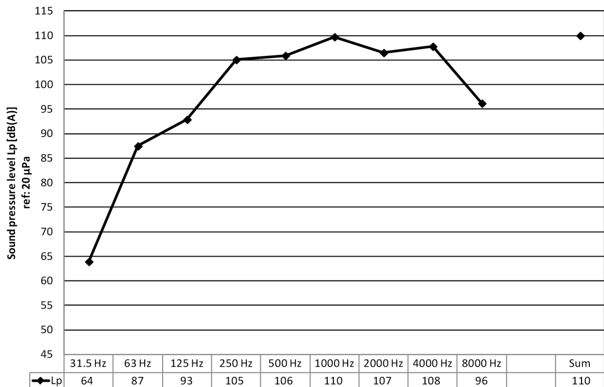
Figure 36: Airborne noise – Sound pressure level L_p – Octave level diagram
