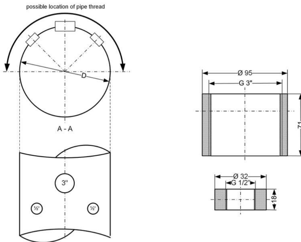
Figure 35: Sampling point, details
