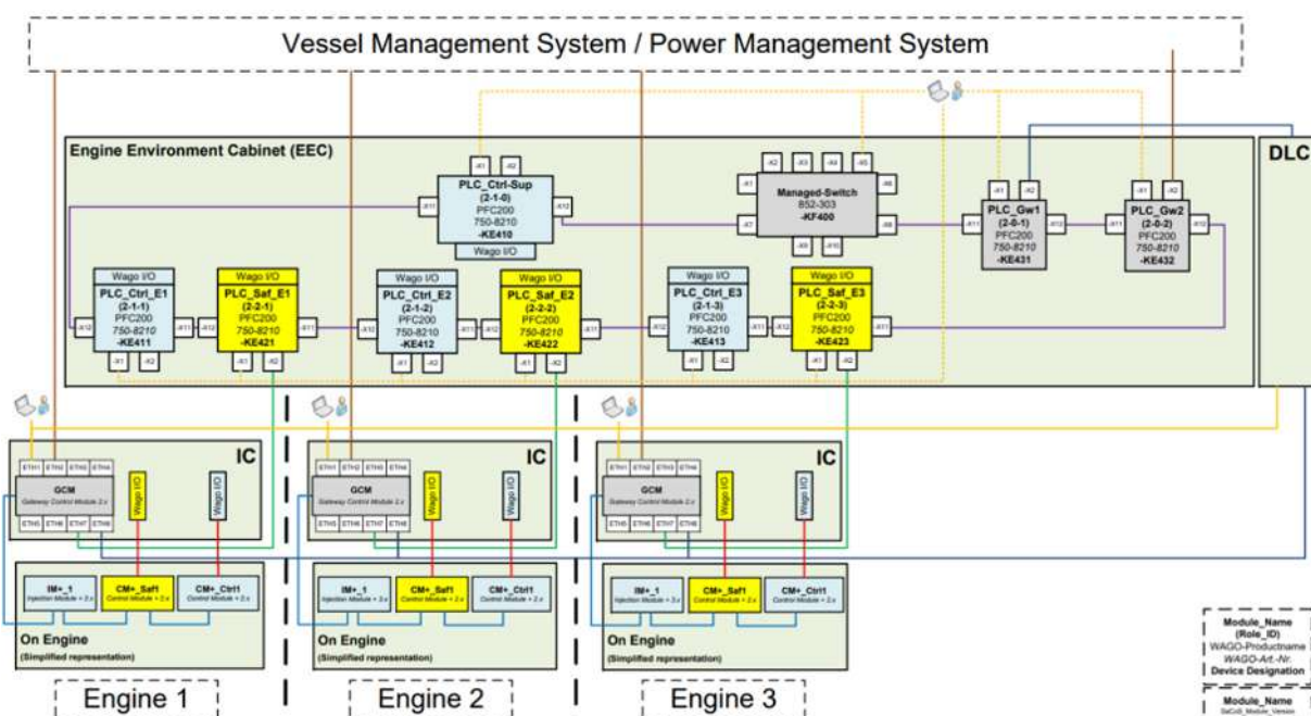
Figure 75: SaCoS ERA system architecture (example for three engines)
