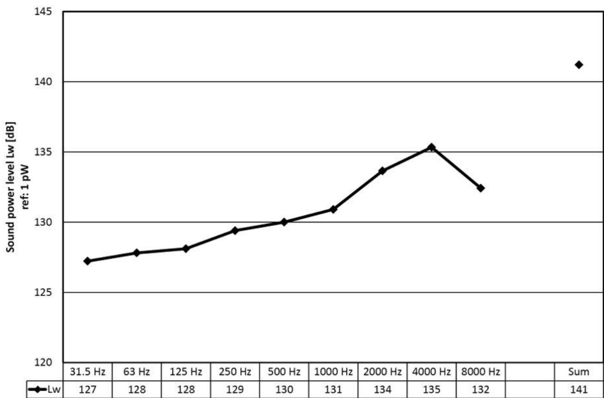
Figure 39: Unsilenced charge air blow-off noise – Sound power level L_w – Octave level diagram
