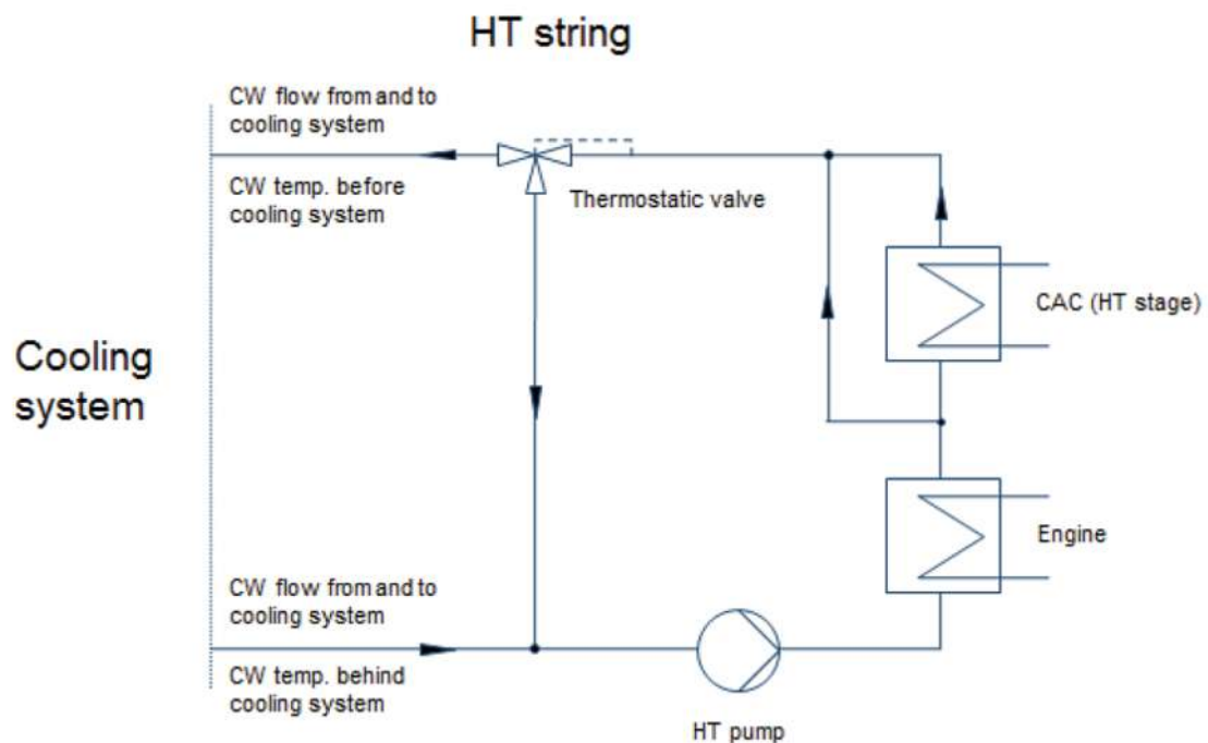
Figure 31: Flow scheme HT string
