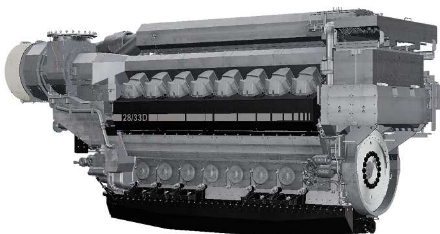
Figure 9: Engine overview, lube oil module with duplex filter, engine view on coupling side (CS)
