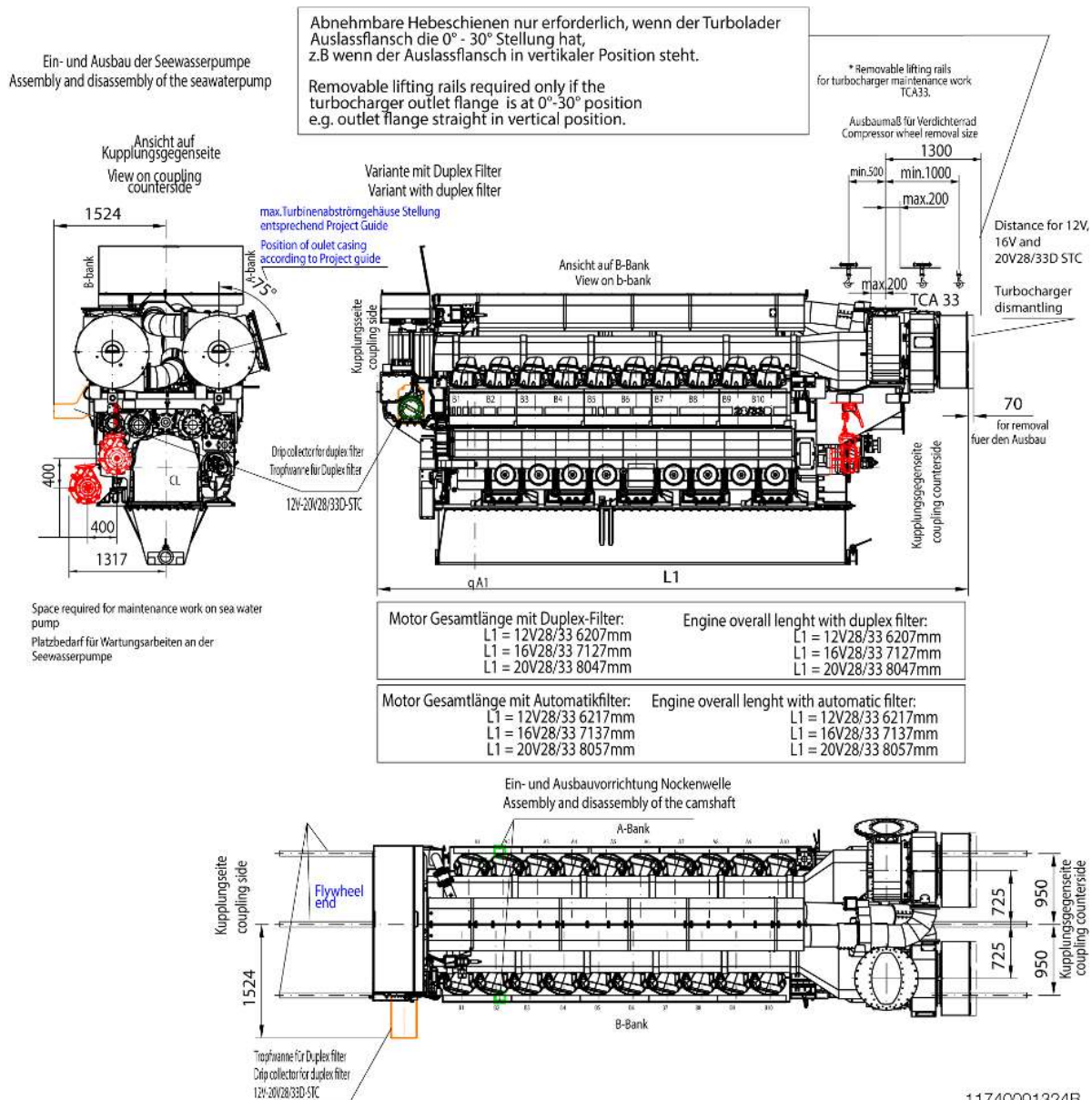
Figure 98: Removal dimensions of lube oil duplex filter, lube oil automatic filter, centrifuge, turbocharger, compressor wheel and seawater pump
