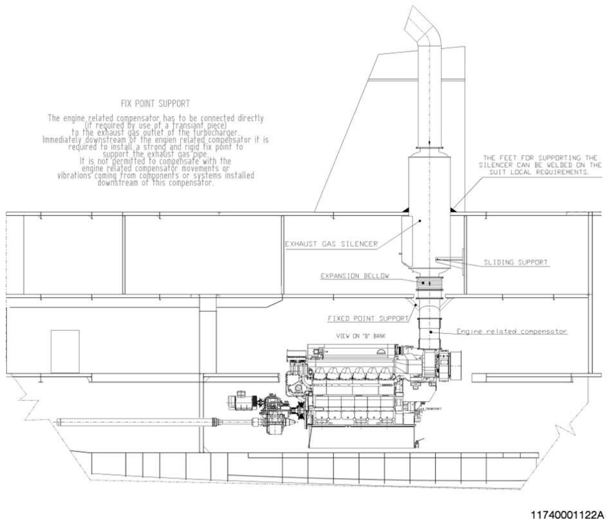
Figure 106: Example: Mechanical propulsion system arrangement – Exhaust gas section
