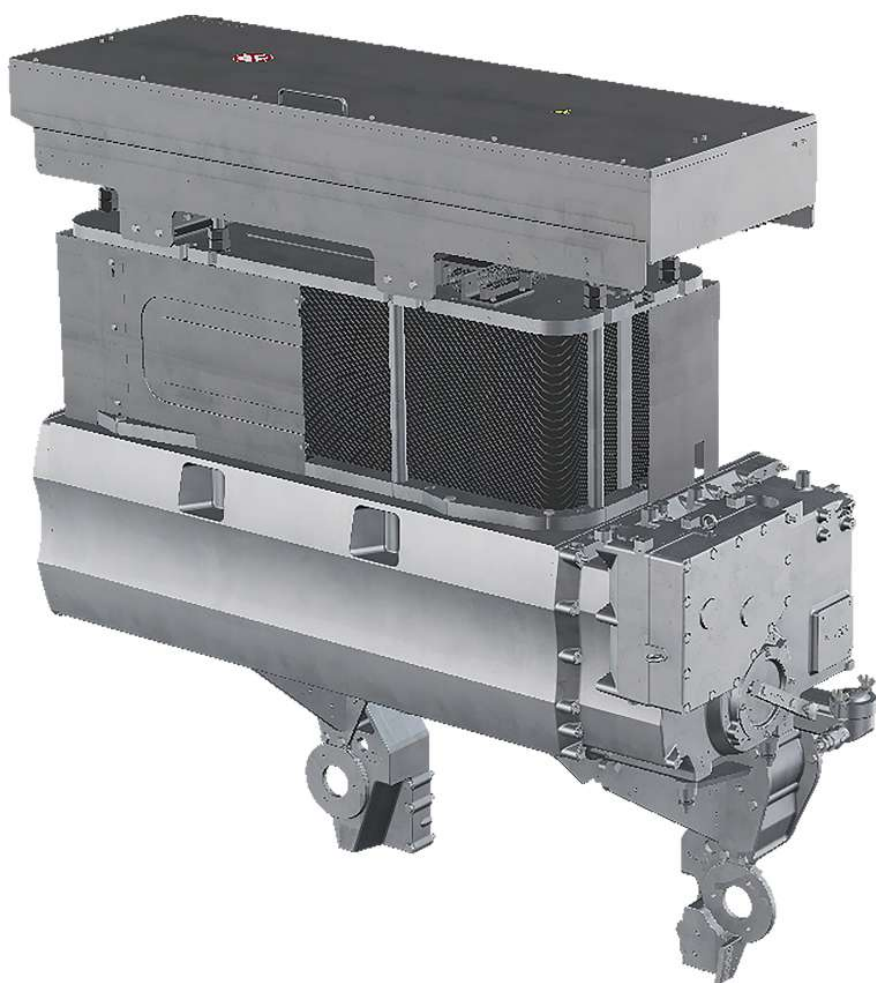
Figure 2: Oil cooler with mounted lube oil duplex filter
