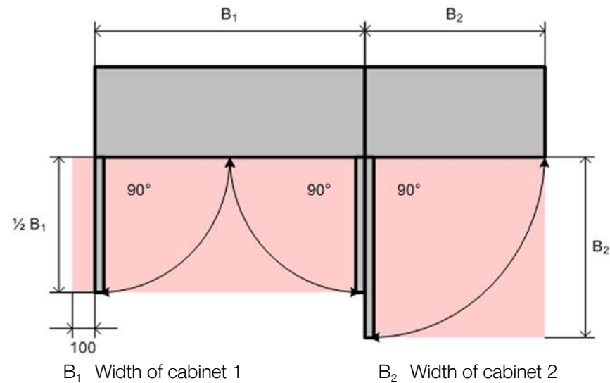
Figure 63: Exemplary arrangement of control cabinets with door opening areas (top view)
