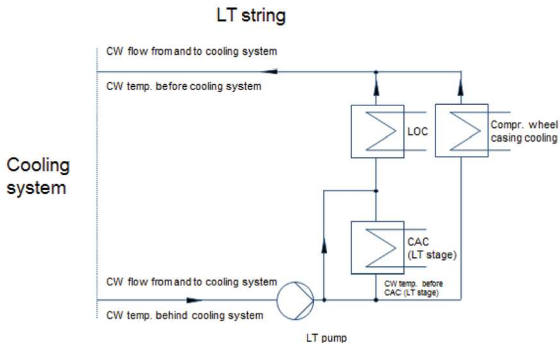
Figure 30: Flow scheme LT string
