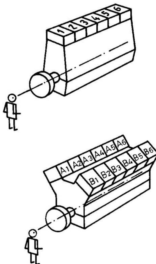
Figure 117: Designation of cylinders
