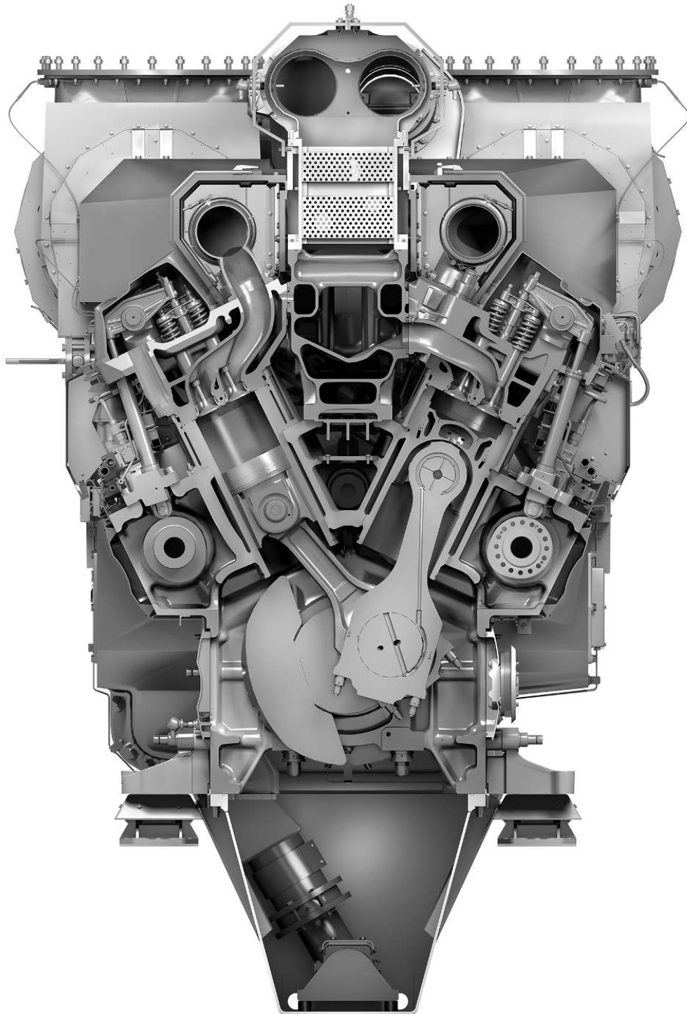
Figure 12: Cross section
