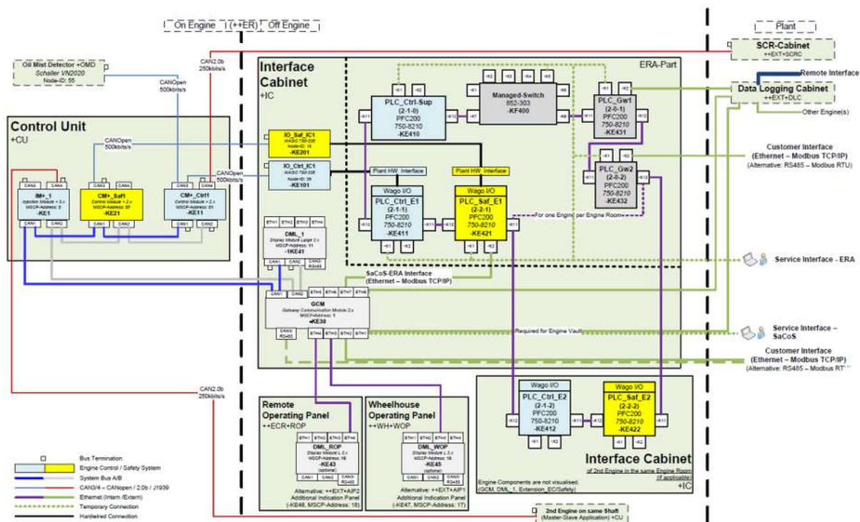
Figure 47: System bus
