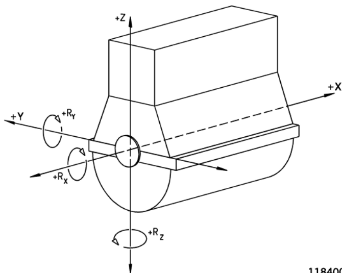
Figure 69: Coordinate system
