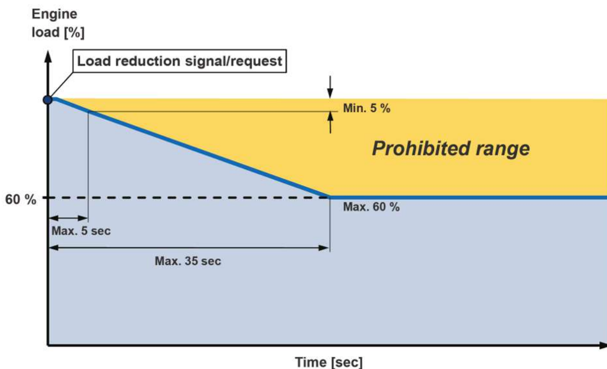
Figure 22: Engine load reduction as a protective safety measure
