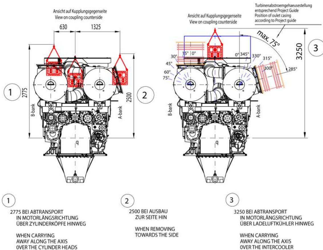
Figure 96: Removal dimensions of charge air cooler bundle
