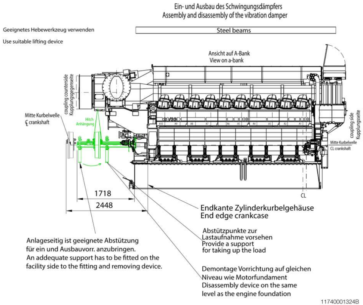
Figure 100: Removal dimensions of vibration damper
