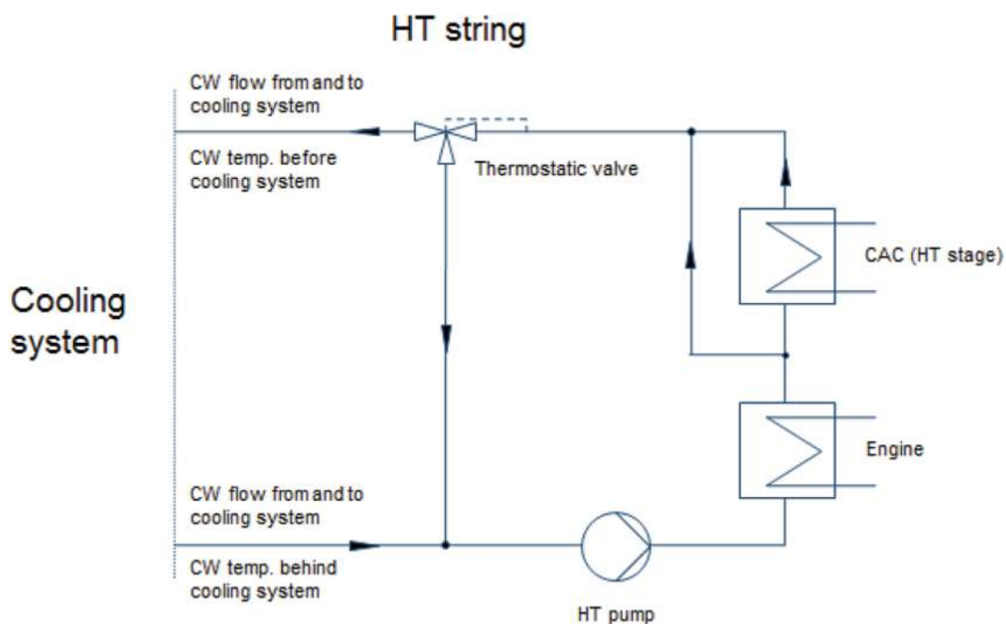
Figure 29: Flow scheme HT string
