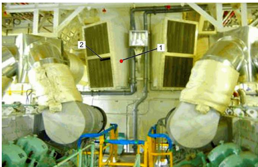
Figure 64: Possible locations for installing the sensor 1TE6000
