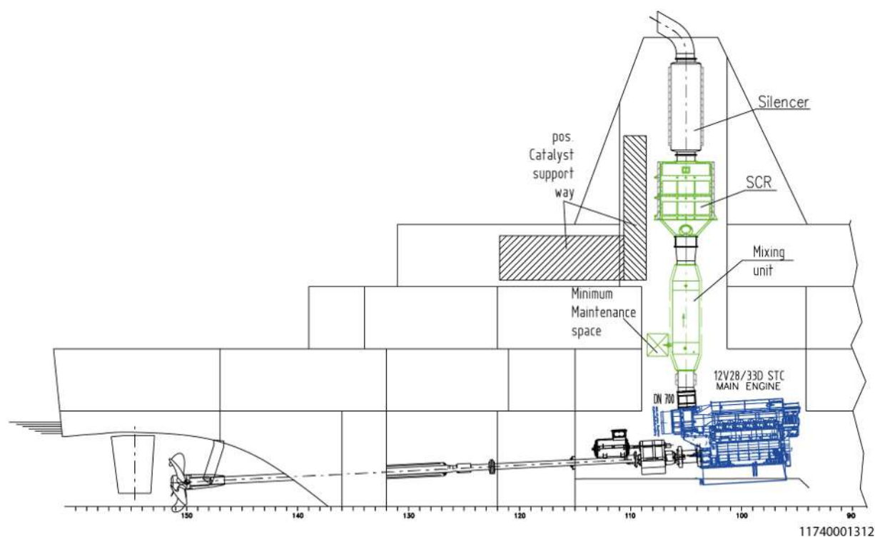
Figure 107: Example: Exhaust gas ducting arrangement
