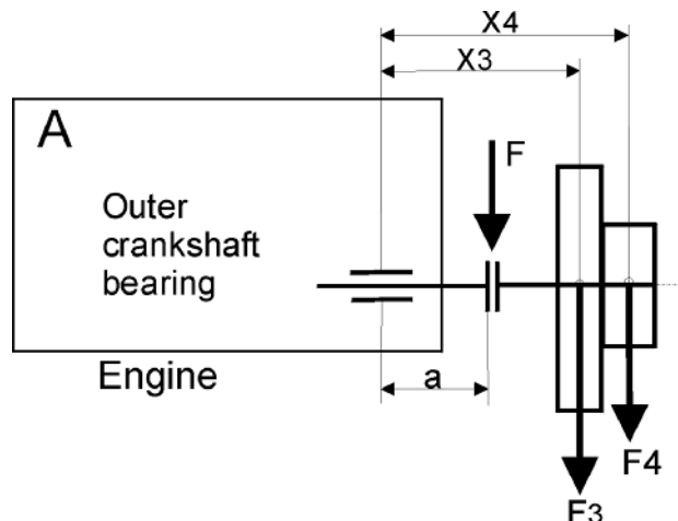
Figure 41: Case A: Overhung arrangement
