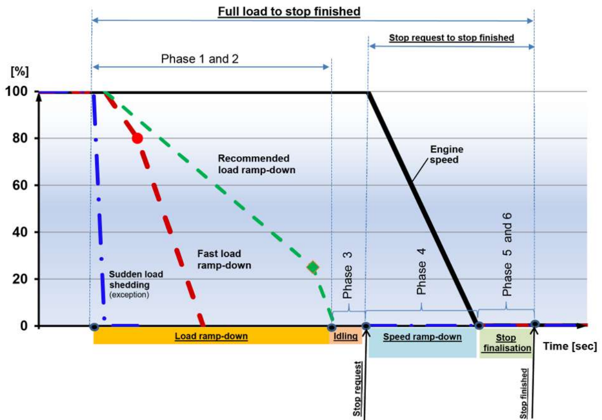
Figure 21: Engine ramping down, generally
