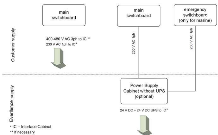
Figure 61: Supply diagram with Power Supply Cabinet
