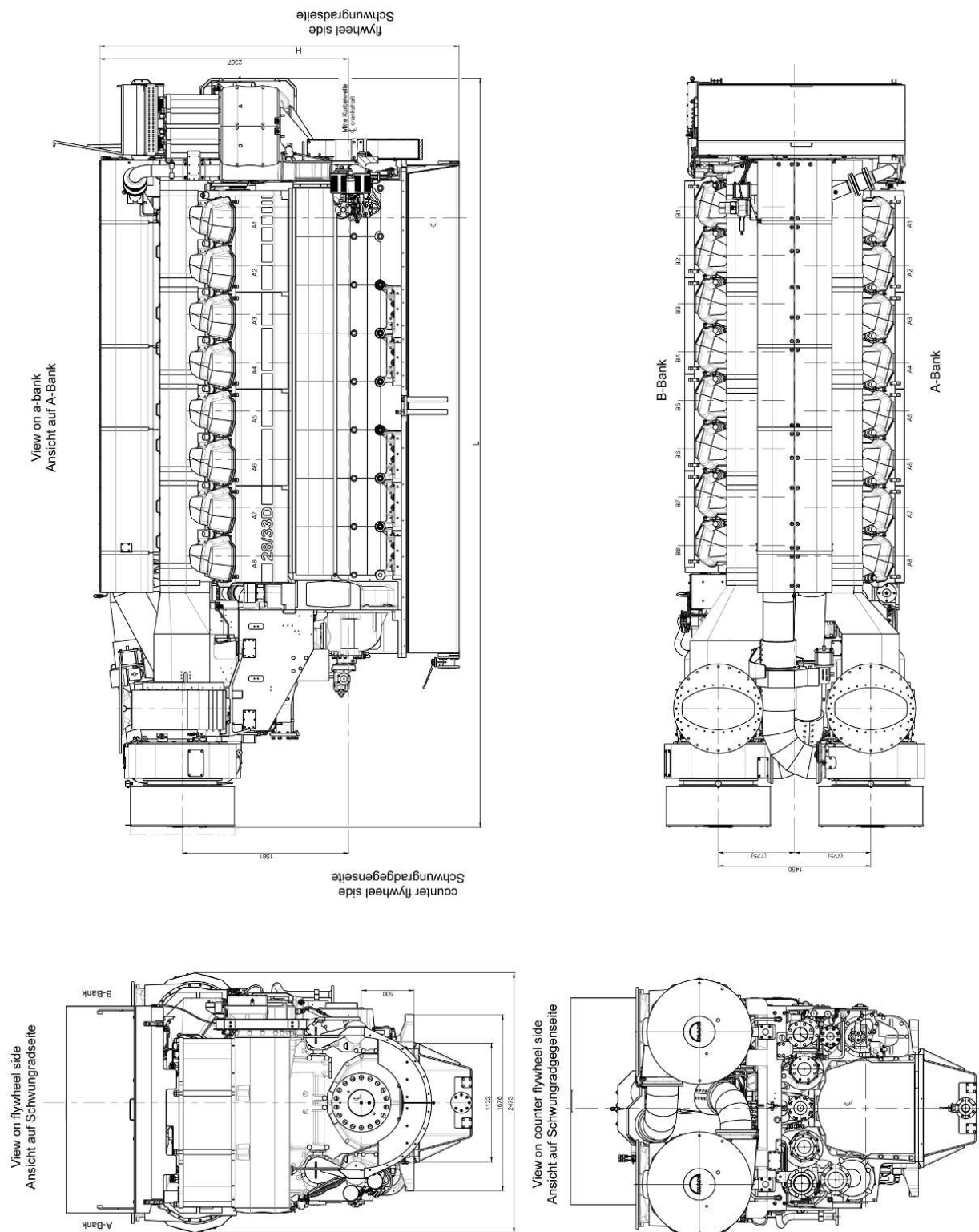
Figure 93: Installation drawing 16V engine with duplex filter (standard) and low oil sump
