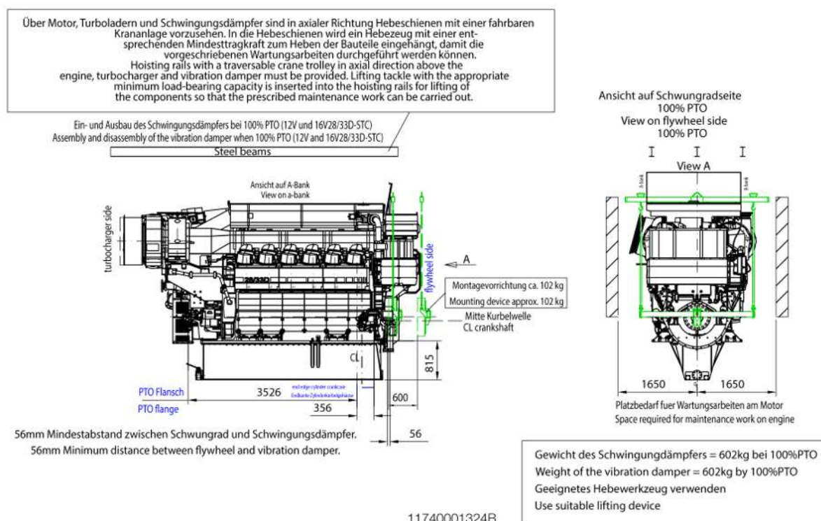
Figure 101: Removal dimensions of vibration damper PTO 100%
