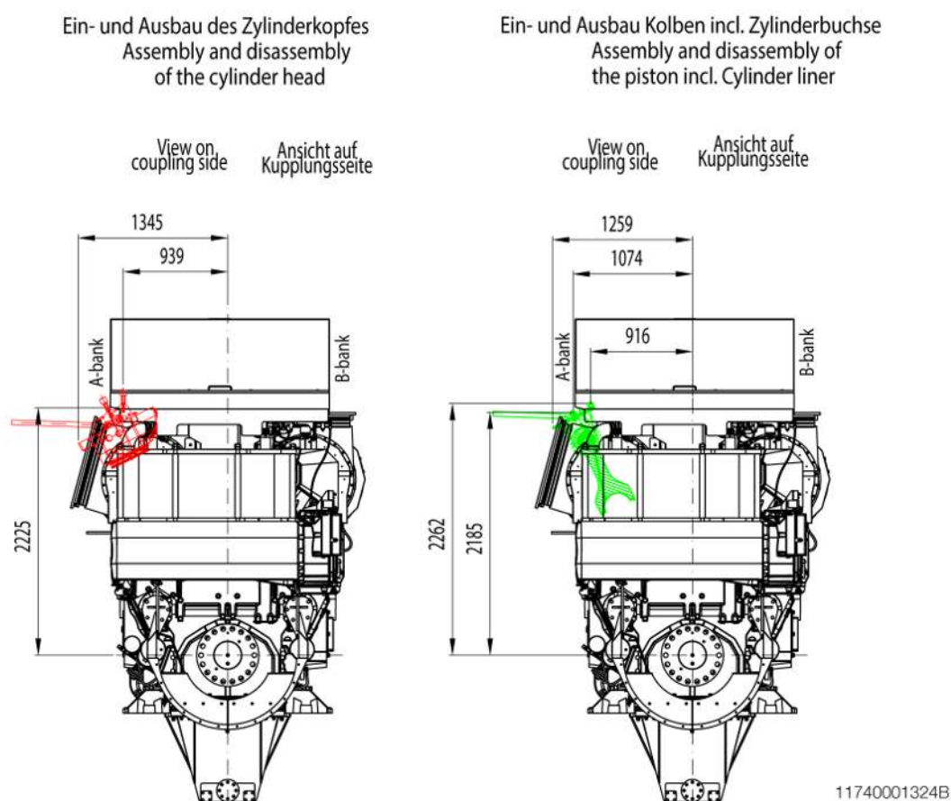
Figure 95: Removal dimensions of cylinder head and piston including cylinder liner
