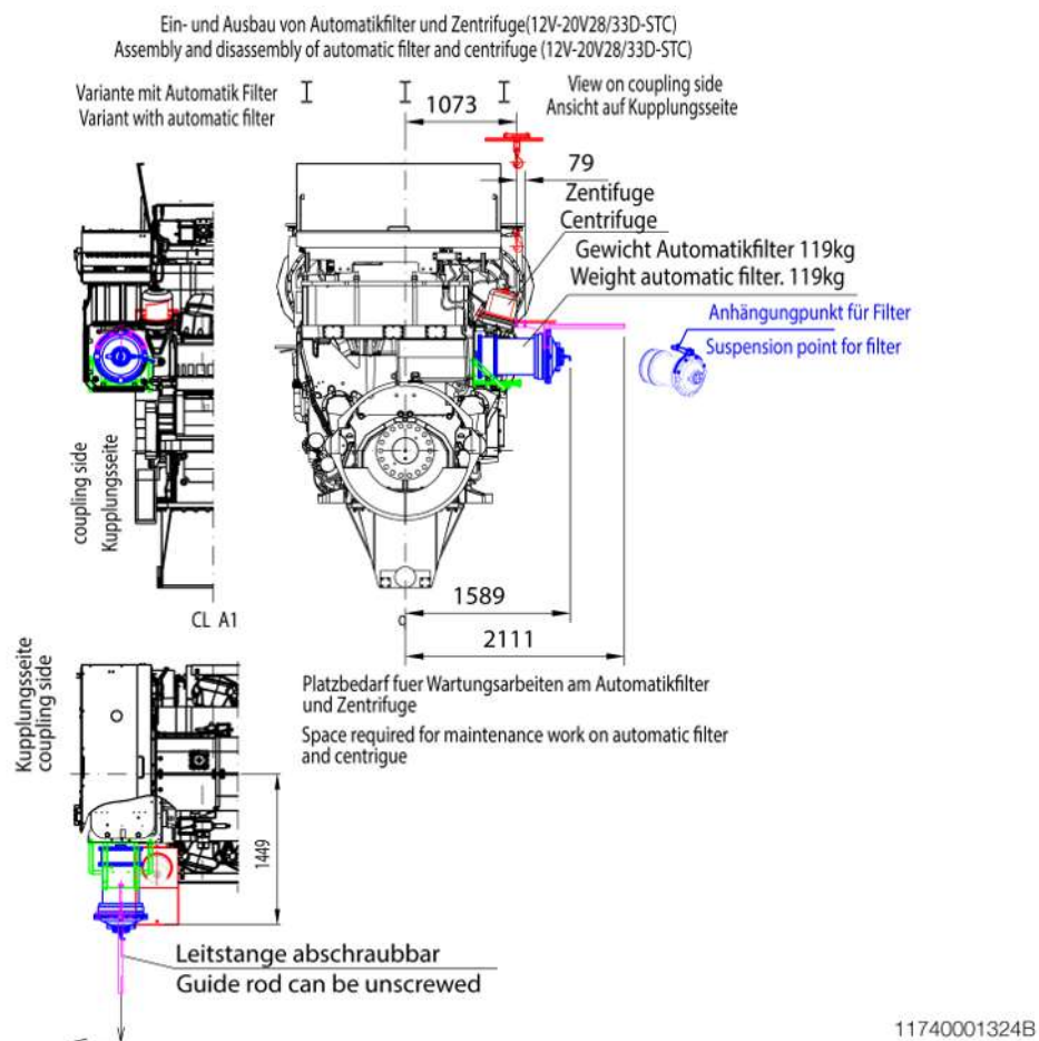
Figure 99: Removal dimensions of seawater pump, lube oil automatic filter, centrifuge, camshaft and turbocharger
