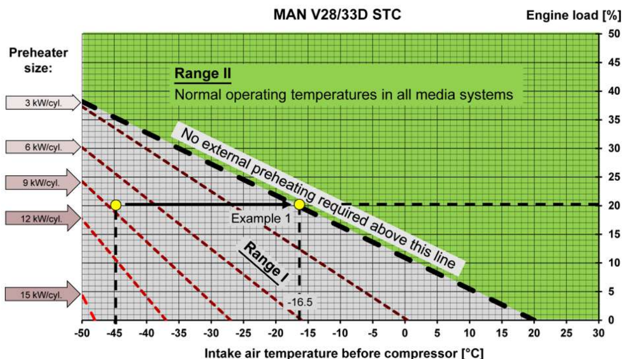
Figure 23: Required preheater size to avoid heat extraction from HT system
