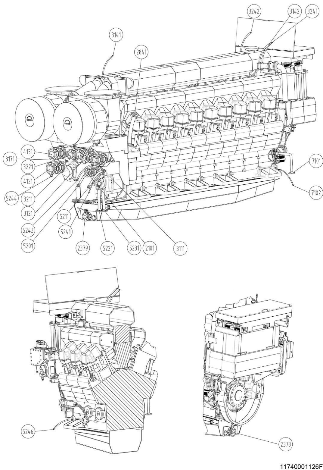
Figure 72: Example of installation of hoses
