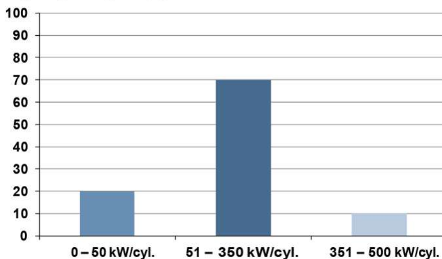
Figure 19: Exemplary load profile: V28/33D STC "Navy" (ICFN), 500 kW/cyl.
