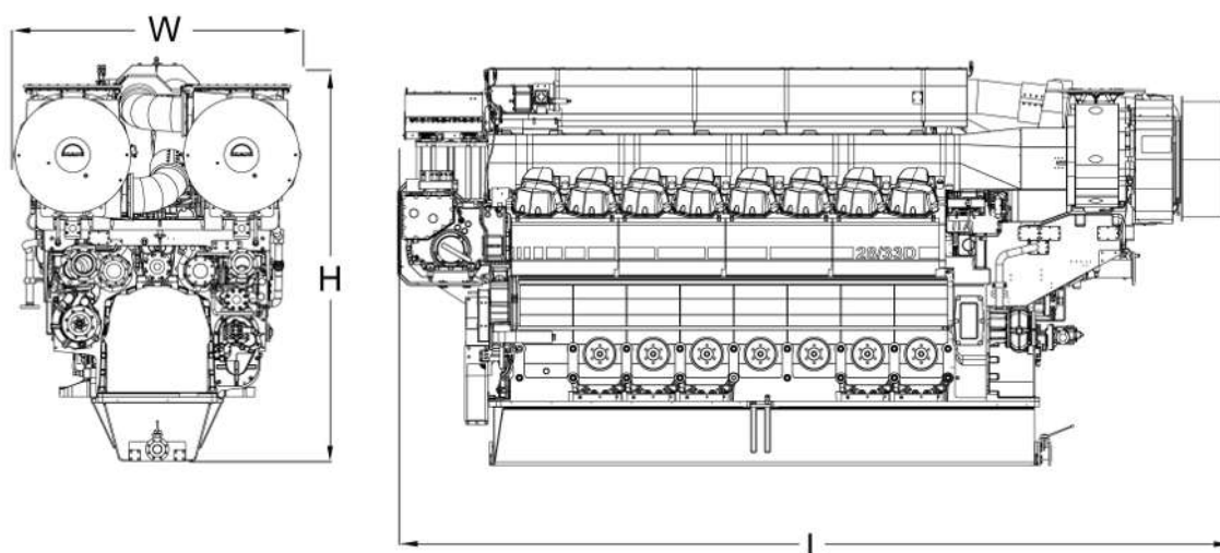
Figure 14: Main dimensions and weights – V28/33D STC mechanical propulsion (lube oil module with duplex filter)
